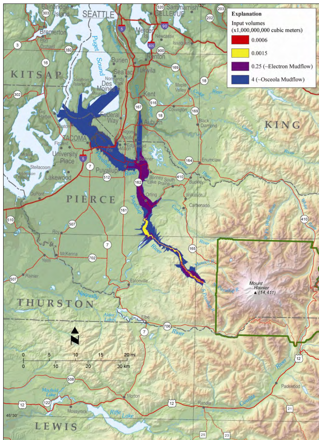
Figure 3. Results of our LAHARZ runs for the Puyallup River. For each user-specified lahar input volume, LAHARZ calculates a cross-sectional area and a planimetric area (shown here) (Iverson and others, 1998; Schilling and others, 2008). The input volumes reported in Iverson (1998) are representative of the various lahar types (Osceola, Electron, and National Mudflows, Case M, Case I, and Case II, respectively).
