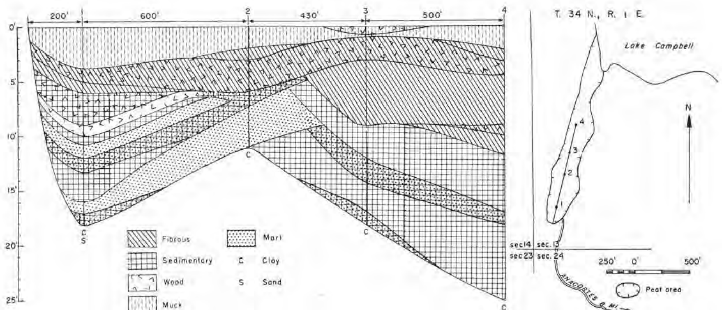
FIGURE 172.—Map and profile of Lake Campbell peat area (27 acres). Map adapted from U. S. Soil Conservation Service soil map.
