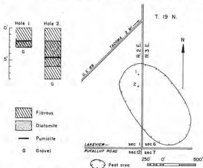
FIGURE 154.—Map and graphic logs of two holes in McChord Airfield peat area (22 acres). Map adapted from U. S. Department of Agriculture soil map of Pierce County.
