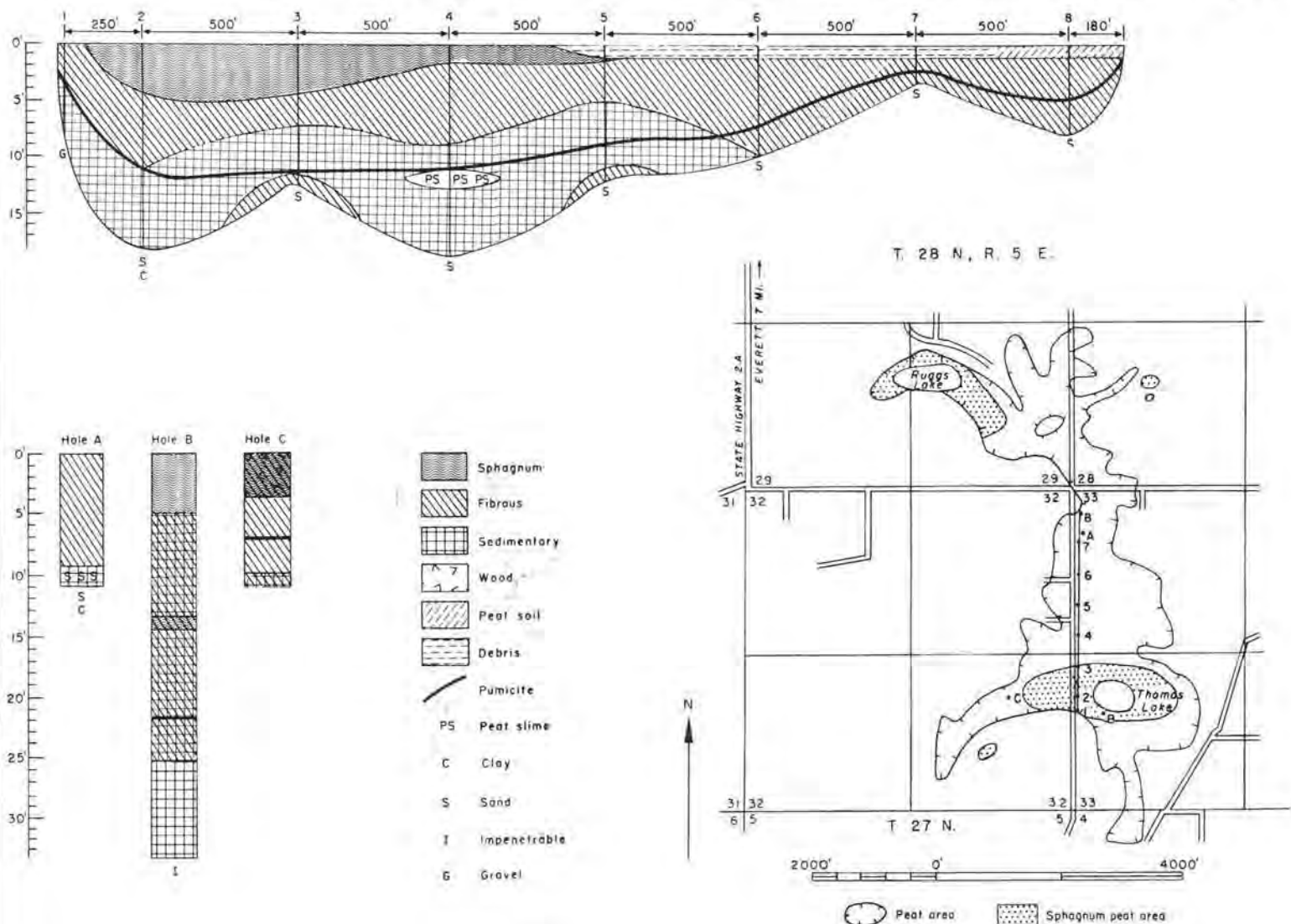
FIGURE 179.—Map, profile, and graphic logs of three holes in Thomas Lake peat area (280 acres). Map adapted from U. S. Department of Agriculture soil map of Snohomish County.
