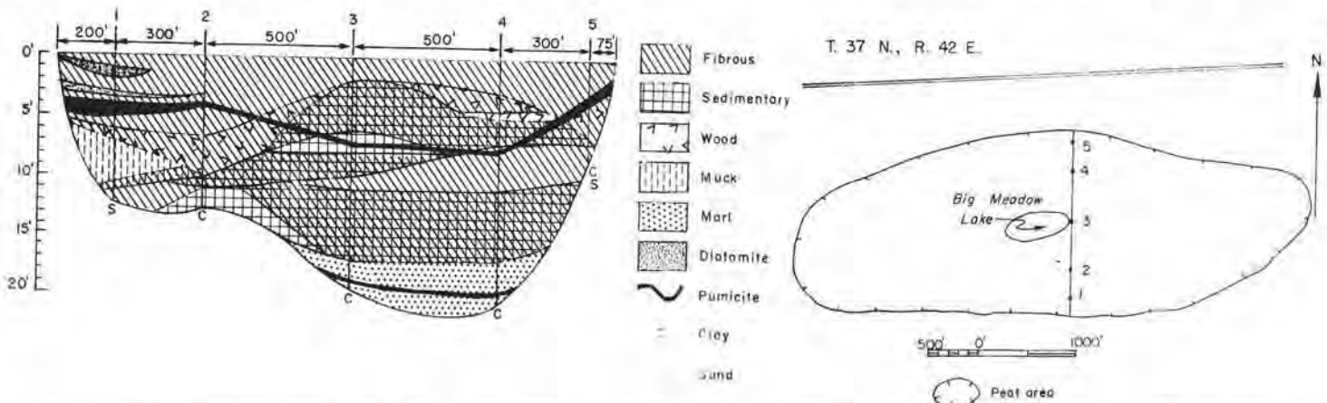
FIGURE 133.—Map and profile of Big Meadow peat area (approximately 170 acres). Map adapted from field sketch.
