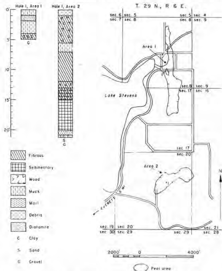
FIGURE 186.—Map and graphic logs of two holes in Lake Stevens peat areas (82 acres and 65 acres). Map adapted from U. S. Department of Agriculture soil map of Snohomish County and U. S. Army Map Service photomosaic.
