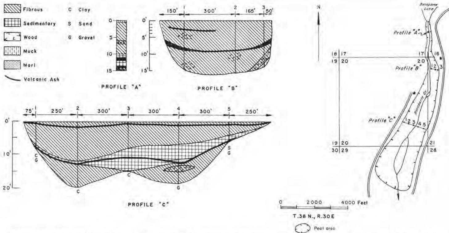
FIGURE 117.—Map, profiles, and graphic log of a hole in Bonaparte Meadows peat area (282 acres). Map adapted from U. S. Geological Survey topographic map (Osoyoos quadrangle).
