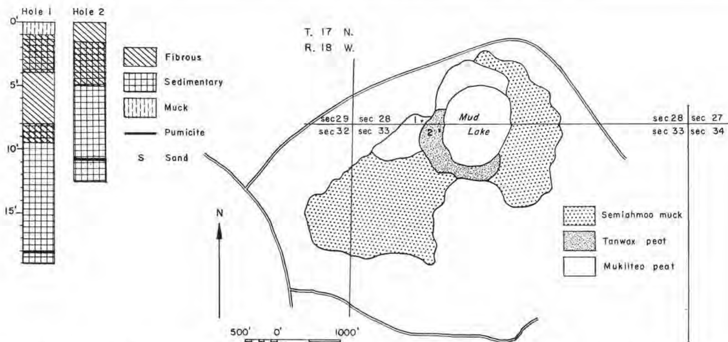
FIGURE 142.—Map and graphic logs of two holes in Mud Lake peat and muck deposit (135 acres). Map adapted from U. S. Department of Agriculture soil map of Pierce County.
