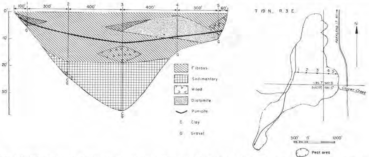
FIGURE 144.—Map and profile of Clover Creek peat area (120 acres). Map adapted from U. S. Department of Agriculture soil map of Pierce County and U. S. Army Map Service photomosaic.
