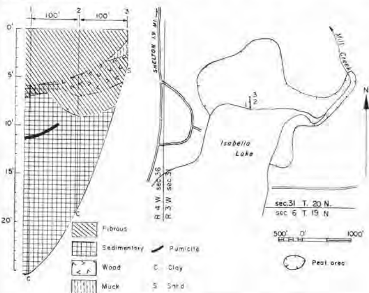
FIGURE 106.—Map and profile of Isabella Lake peat area (69 acres). Map adapted from U. S. Department of Agriculture unpublished soil map of Mason County and U. S. Army Map Service photomosaic.
