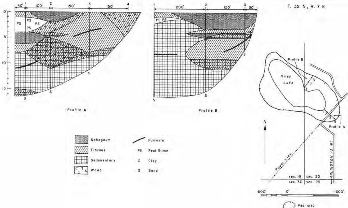
FIGURE 189.—Map and profiles of Riley Lake peat area (38 acres). Map adapted from U. S. Department of Agriculture soil map of Snohomish County and U. S. Army Map Service photomosaic.
