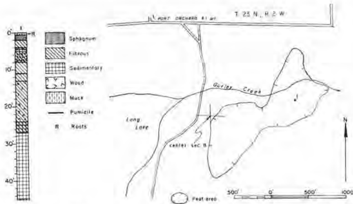
FIGURE 89.—Map and graphic log of a hole in Gurley Creek peat area (23 acres). Map adapted from U. S. Department of Agriculture soil map of Kitsap County.
