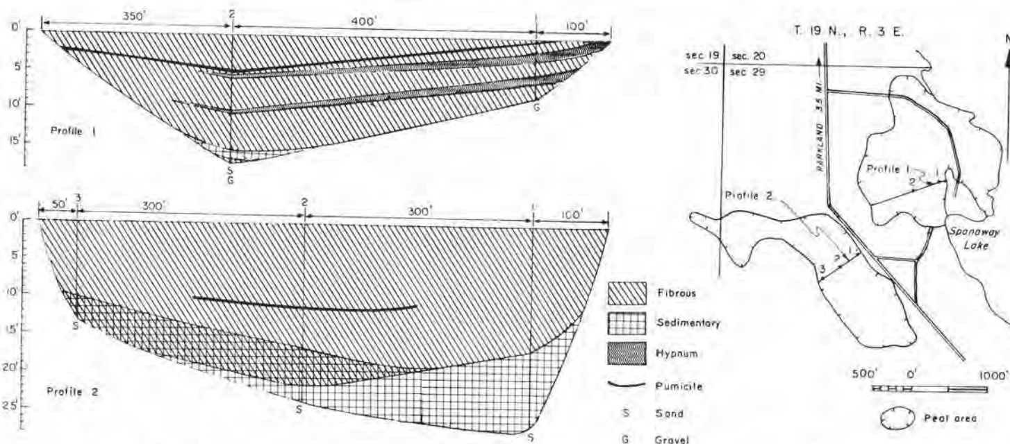
FIGURE 147.—Map and profiles of Spanaway Lake peat areas (54 acres and 46 acres). Map adapted from U. S. Department of Agriculture soil map of Pierce County.
