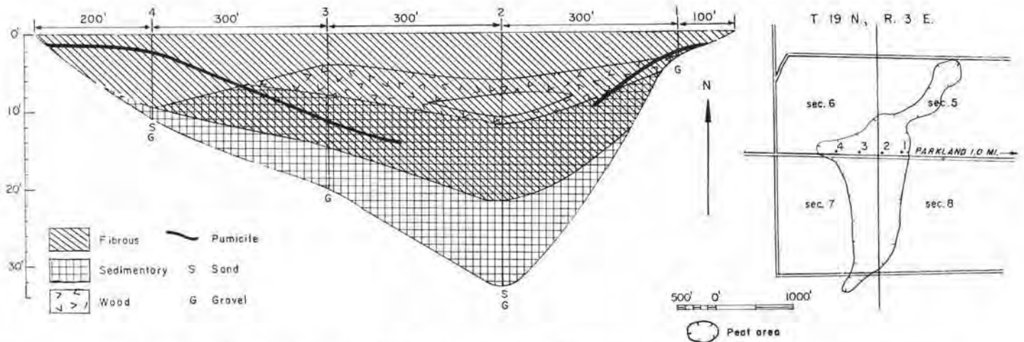
FIGURE 151.—Map and profile of Parkland peat area (38 acres). Map adapted from U. S. Department of Agriculture soil map of Pierce County.
