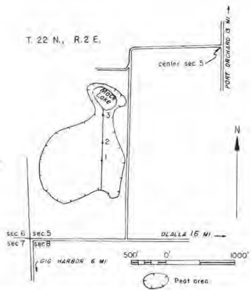
FIGURE 88.—Map and profile of Mace Lake peat area (29 acres). Map adapted from U. S. Army Map Service photomosaic.
