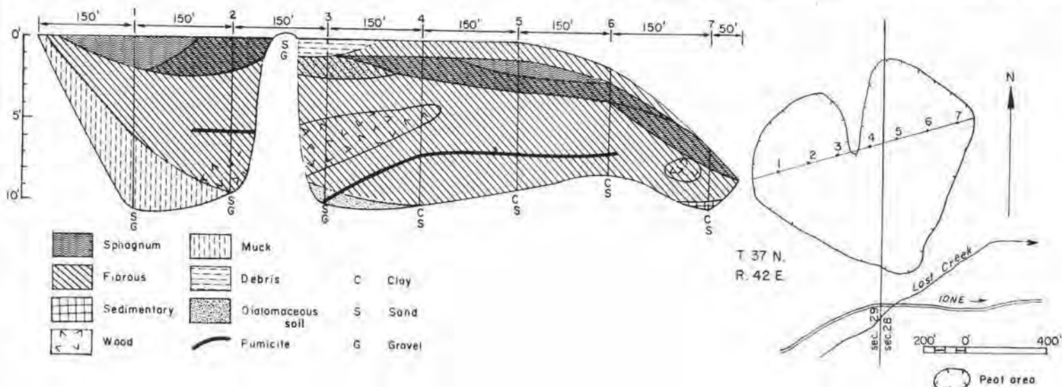
FIGURE 136.—Map and profile of Lost Creek peat area (5 acres). Map adapted from field sketch.
