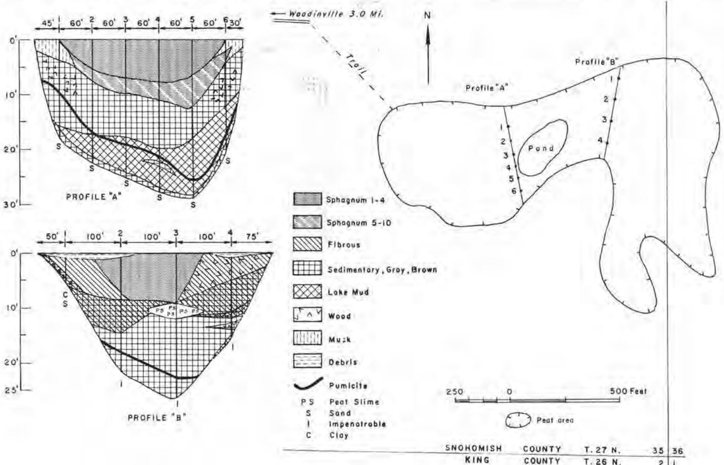
FIGURE 190.—Map and profiles of Hooven peat area (20 acres). Map adapted from U. S. Department of Agriculture soil map of Snohomish County, U. S. Army Map Service photomosaic, and Rigg and Richardson (1938).
