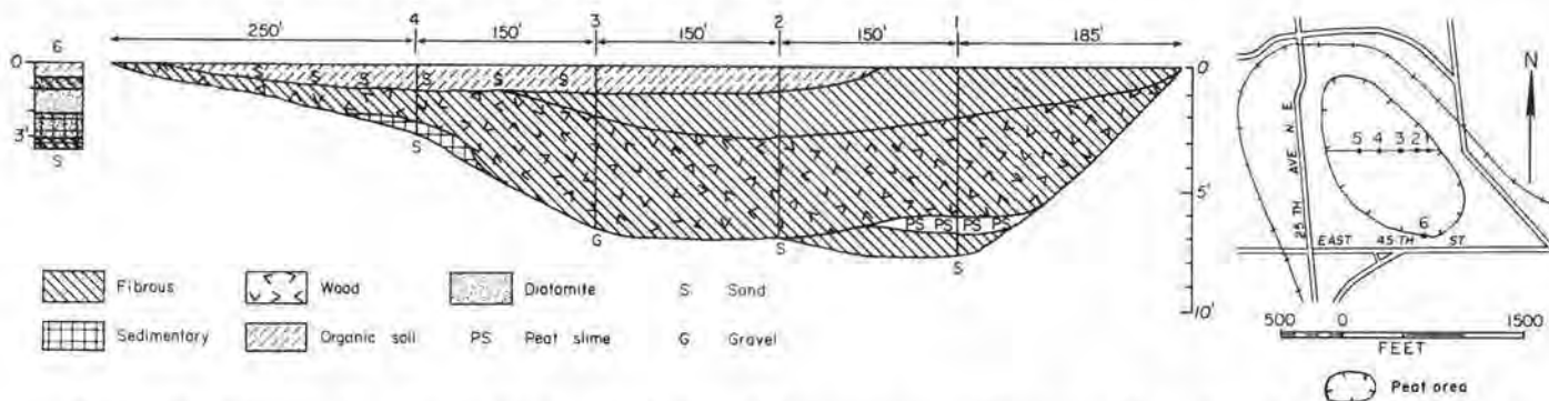
FIGURE 62.—Map, profile, and graphic log of a hole in Malmo peat area (24 acres). Map adapted from field sketch.
