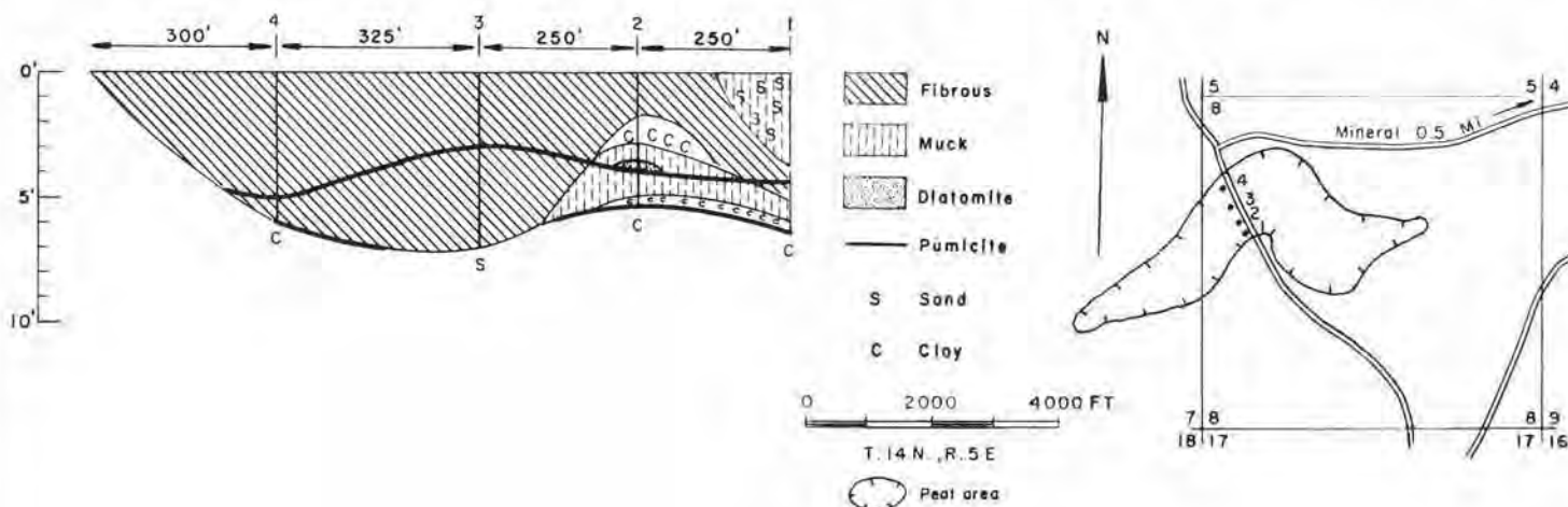
FIGURE 101.—Map and profile of Mineral peat area (148 acres). Map adapted from U. S. Department of Agriculture soil map of Lewis County.
