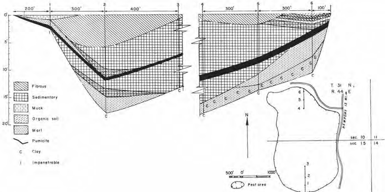
FIGURE 129.—Map and profile of Kent Meadows peat area (175 acres). Map adapted from U. S. Soil Conservation Service soil map.
