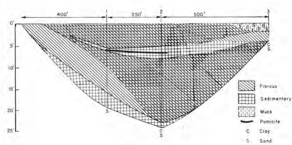
FIGURE 87.—Map and profiles of Lost Lake peat area (30 acres). Map adapted from U. S. Army Map Service photomosaic.
