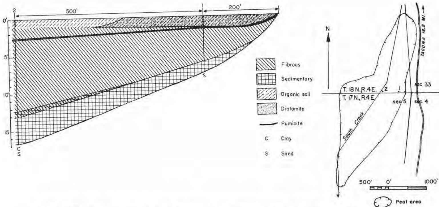
FIGURE 143.—Map and profile of South Creek peat area (132 acres). Map adapted from U. S. Department of Agriculture soil map of Pierce County.
