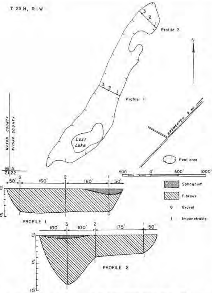
FIGURE 87.—Map and profiles of Lost Lake peat area (30 acres). Map adapted from U. S. Army Map Service photomosaic.
