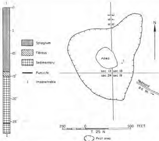
FIGURE 72.—Map and graphic log of a hole in Ames Lake peat area (10 acres). Map adapted from U. S. Department of Agriculture soil map of King County and U. S. Army Map Service photomosaic.
