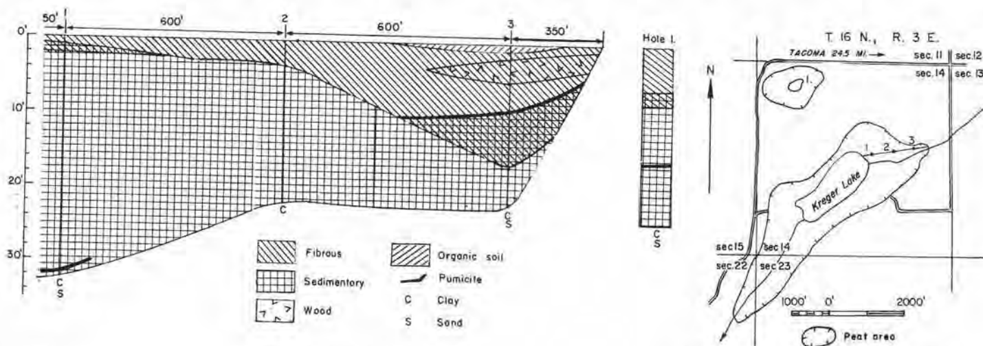
FIGURE 140.—Map, profile, and graphic log of a hole in Kreger Lake peat areas (180 acres and 34 acres). Map adapted from U. S. Department of Agriculture soil map of Pierce County.
