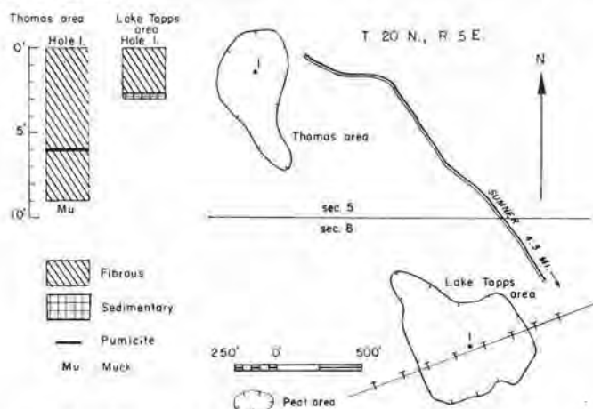
FIGURE 158.—Map and graphic logs of two holes in Lake Tapps and Thomas peat areas (9 acres and 5 acres). Map adapted from U. S. Department of Agriculture soil map of Pierce County.
