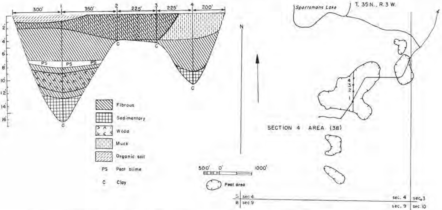
FIGURE 161.—Map and profile of Section 4 peat area (40 acres). Map adapted from field sketch by John Sherman.
