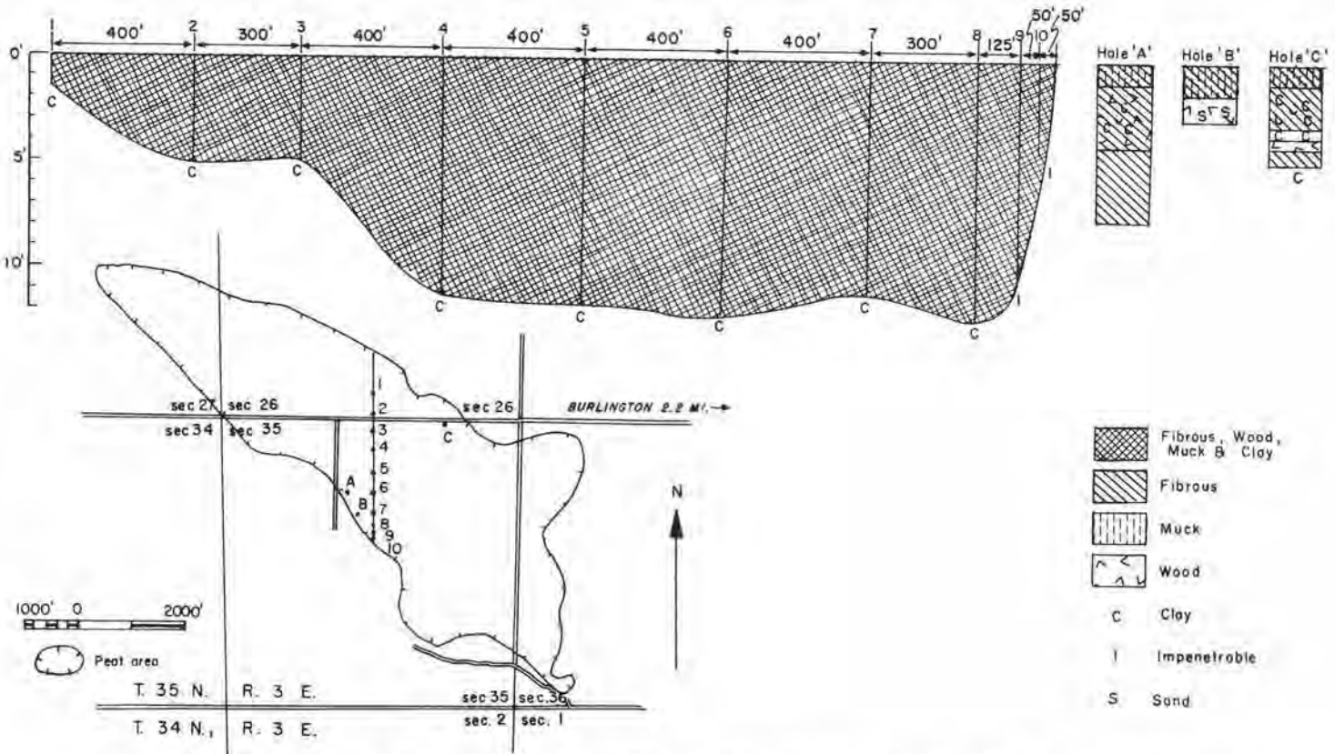
FIGURE 167.—Map, profile, and graphic logs of three holes in Burlington peat area (616 acres). Map adapted from U. S. Soil Conservation Service soil map.
