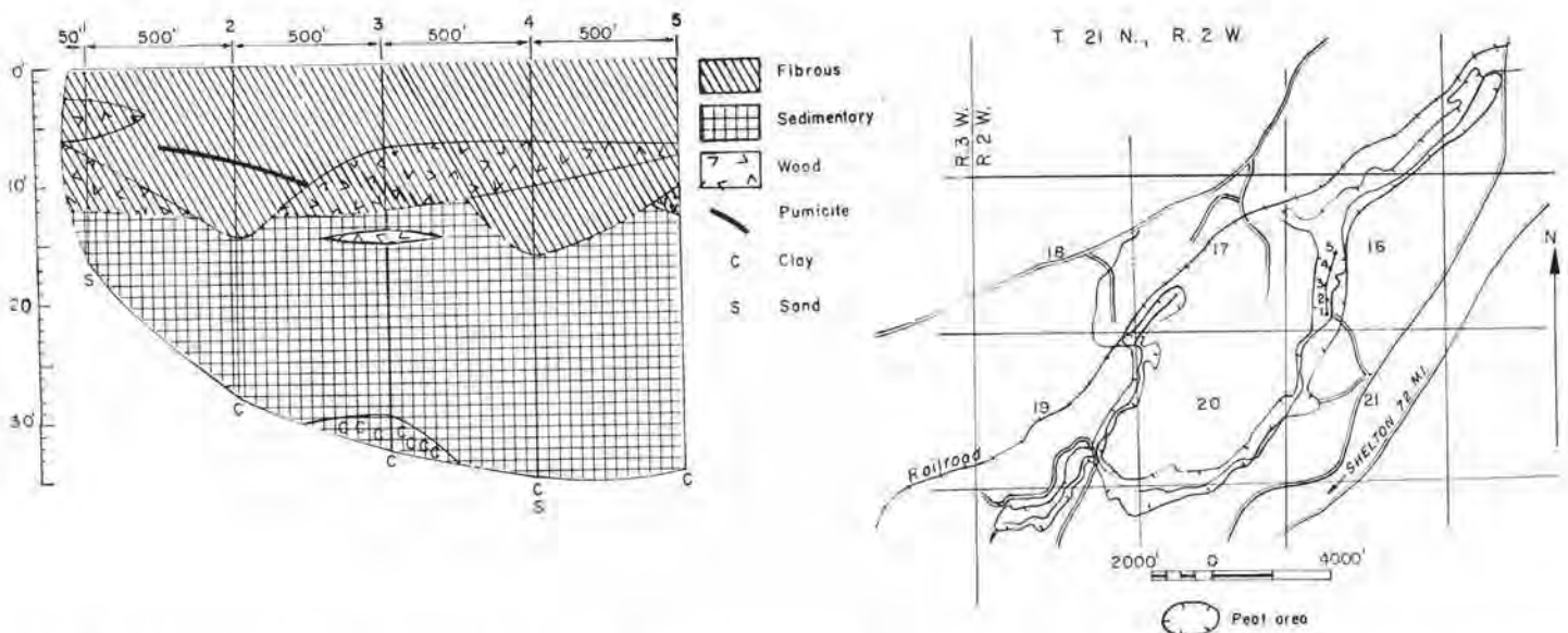
FIGURE 102.—Map and profile of Deer Creek peat area, Mason County (500 acres). Map adapted from U. S. Department of Agriculture unpublished soil map of Mason County.
