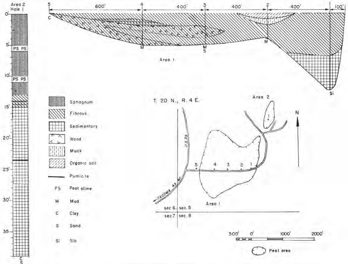
FIGURE 148.—Map, profile, and graphic log of a hole in Milton peat areas (53 acres and 5 acres). Map adapted from U. S. Department of Agriculture soil map of Pierce County.
