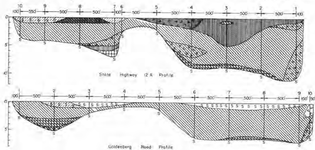
FIGURE 118.—Map and profiles of Peninsula peat areas, Pacific County (3,000 to 4,000 acres, estimated). Map adapted from U. S. Soil Conservation Service soil map and U. S. Army Map Service photomosaic.
