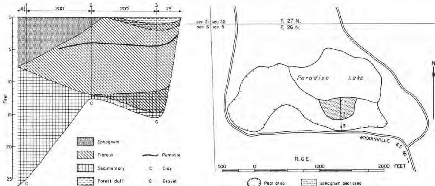
FIGURE 63.—Map and profile of Paradise Lake peat area No. 1, King County (23 acres, including 4 acres of sphagnum). Map adapted from U. S. Department of Agriculture soil map of King County.
