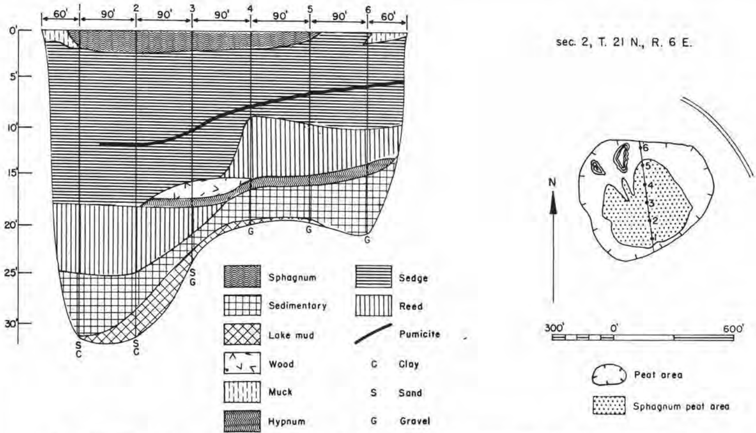
FIGURE 65.—Map and profile of Black Diamond peat area (18 acres). Map adapted from Rigg and Richardson (1938).
