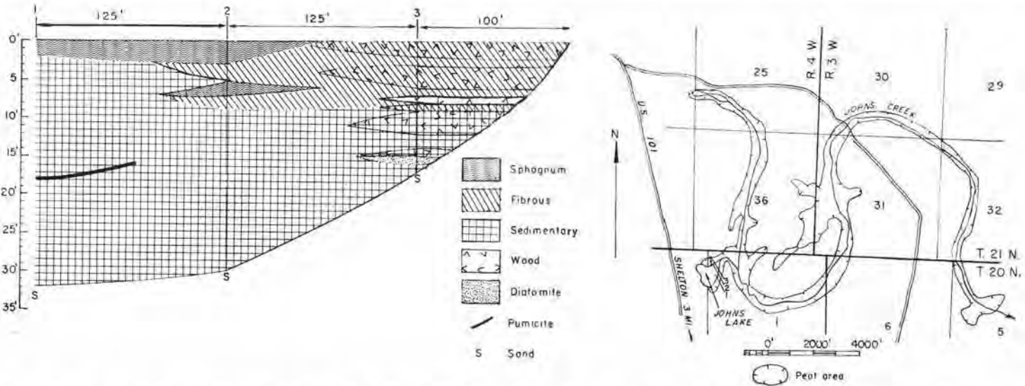
FIGURE 103.—Map and profile of Johns Creek peat area (500 acres). Map adapted from U. S. Department of Agriculture unpublished soil map of Mason County.
