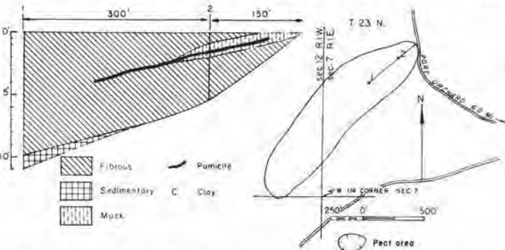
FIGURE 93.—Map and profile of Sunnyslope peat area (13 acres). Map adapted from U. S. Department of Agriculture soil map of Kitsap County and U. S. Army Map Service photomosaic.
