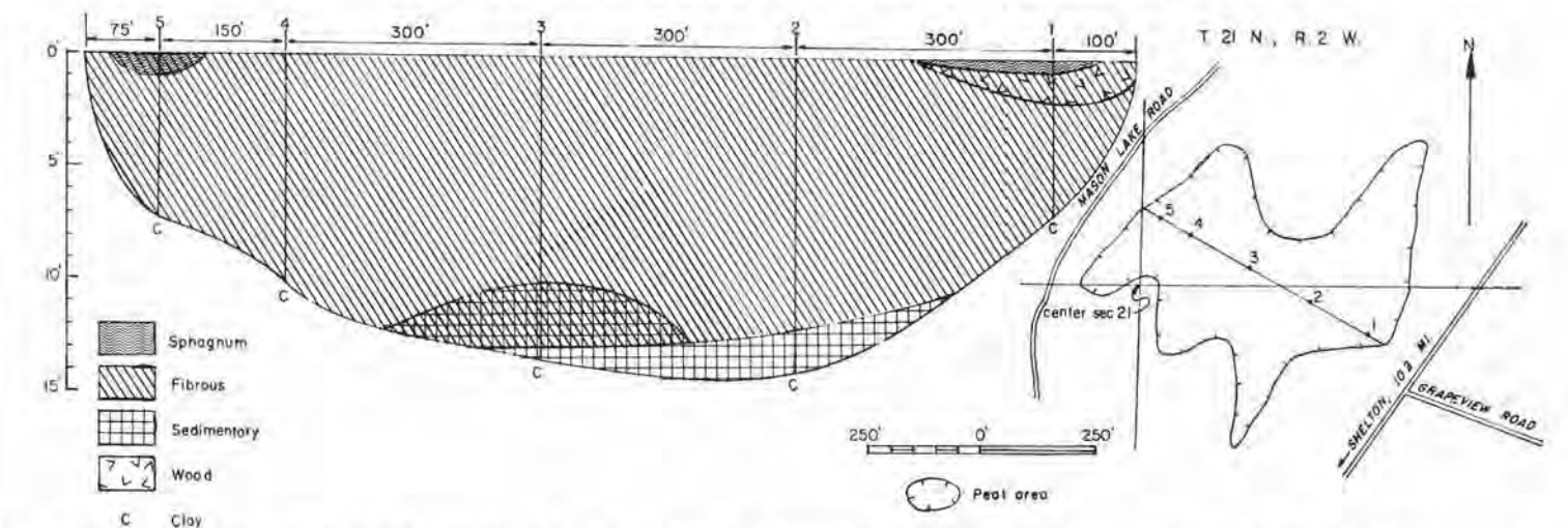
FIGURE 110.—Map and profile of Grapeview Road peat area (24 acres). Map adapted from U. S. Army Map Service photomosaic.
