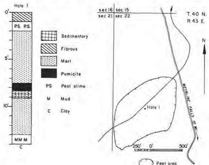
FIGURE 137.—Map and graphic log of a hole in Fence Creek peat area (18 acres). Map adapted from aerial photograph.
