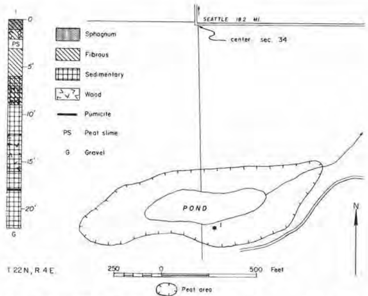
FIGURE 75.—Map and graphic log of a hole in Bingaman Lake peat area (7 acres). Map adapted from U. S. Department of Agriculture soil map of King County and U. S. Army Map Service photomosaic.
