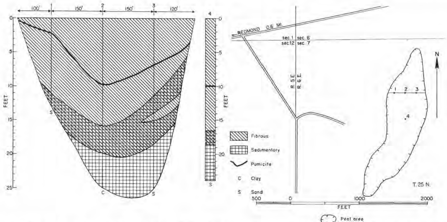
FIGURE 64.—Map, profile, and graphic log of a hole in Redmond peat area (21 acres). Map adapted from U. S. Department of Agriculture soil map of King County and U. S. Army Map Service photomosaic.
