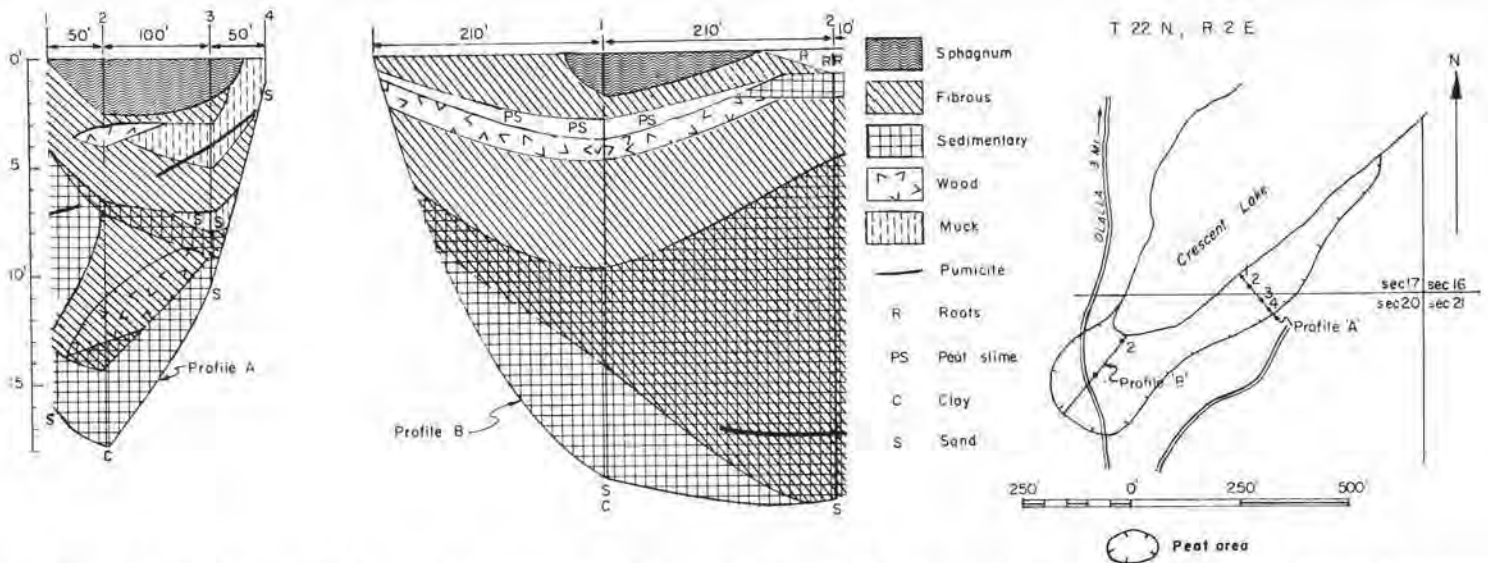
FIGURE 155.—Map and profiles of Crescent Lake peat area No. 1 (10 acres). Map adapted from U. S. Army Map Service photomosaic.
