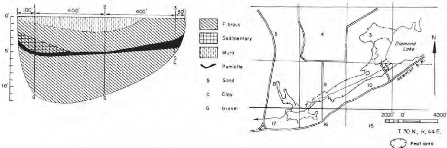
FIGURE 124.—Map and profile of Southwest End Diamond Lake peat area (528 acres). Map adapted from U. S. Soil Conservation Service soil map and aerial photograph.
