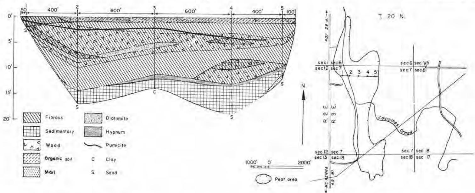
FIGURE 138.—Map and profile of Lacamas Creek peat area (262 acres). Map adapted from U. S. Department of Agriculture soil map of Pierce County.
