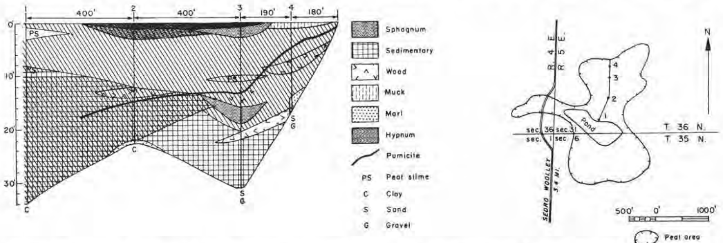
FIGURE 169.—Map and profile of Sedro Woolley peat area (62 acres). Map adapted from U. S. Army Map Service photomosaic.
