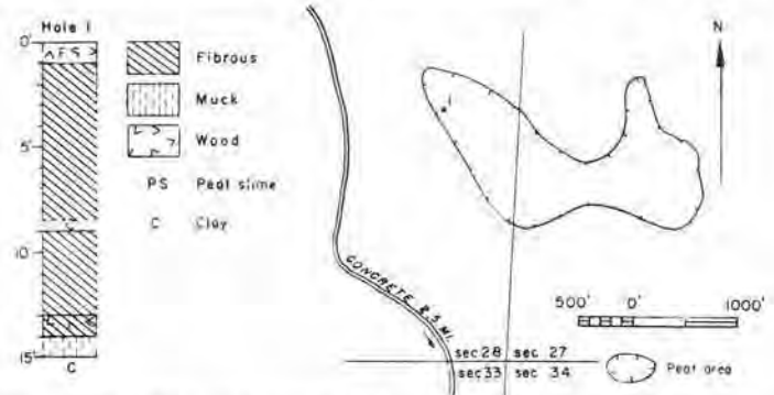
FIGURE 170.—Map and graphic log of a hole in Sawmill peat area (48 acres). Map adapted from U. S. Army Map Service photo-mosaic.
