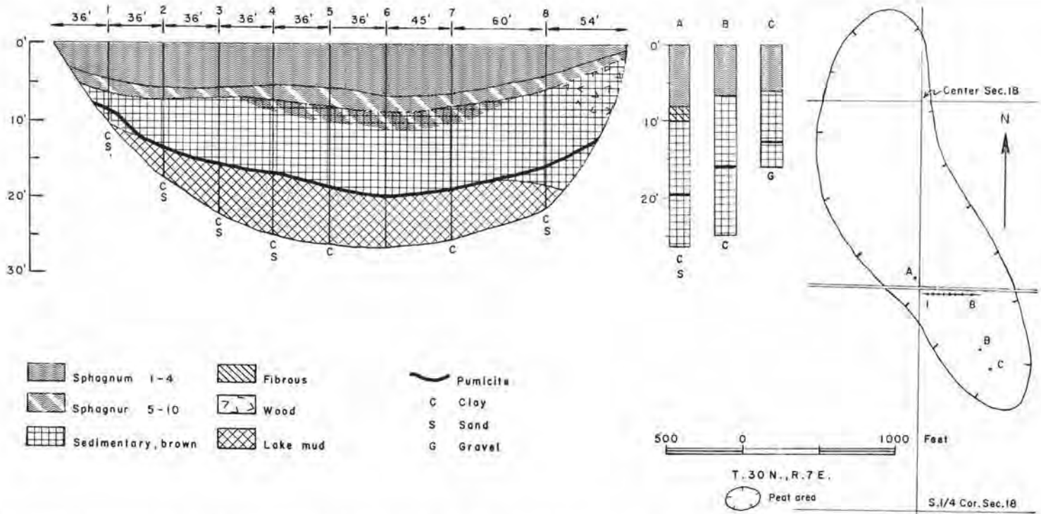
FIGURE 187.—Map, profile, and graphic logs of three holes in Granite Falls peat area (42 acres). Map adapted from U. S. Department of Agriculture soil map of Snohomish County and U. S. Army Map Service photomosaic.
