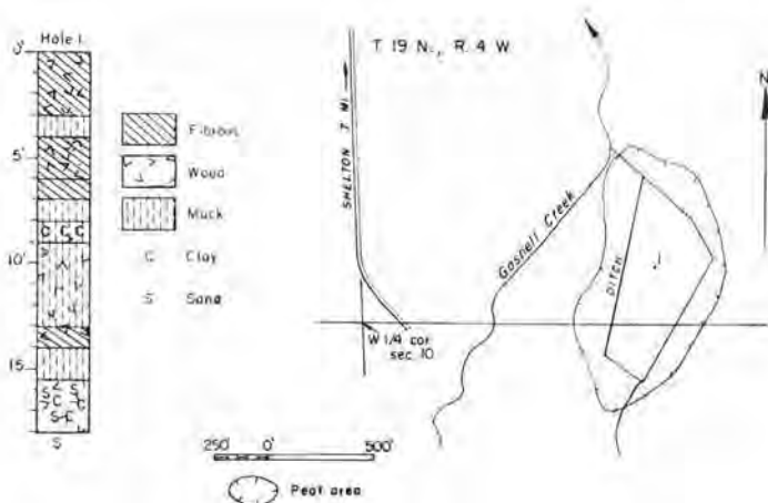
FIGURE 115.—Map and graphic log of a hole in Wivell Farm peat area (13 acres). Map adapted from U. S. Department of Agriculture unpublished soil map of Mason County.
