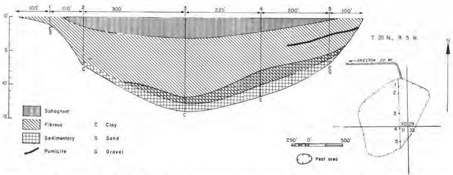
FIGURE 113.—Map and profile of C.C.C. Project Number 5 peat area (19 acres). Map adapted from Simpson Logging Co. map.
