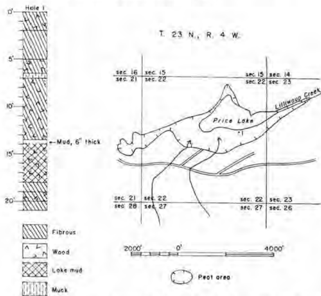
FIGURE 105.—Map and graphic log of a hole in Price Lake peat area (124 acres). Map adapted from U. S. Department of Agriculture unpublished soil map of Mason County and U. S. Army Map Service photomosaic.
