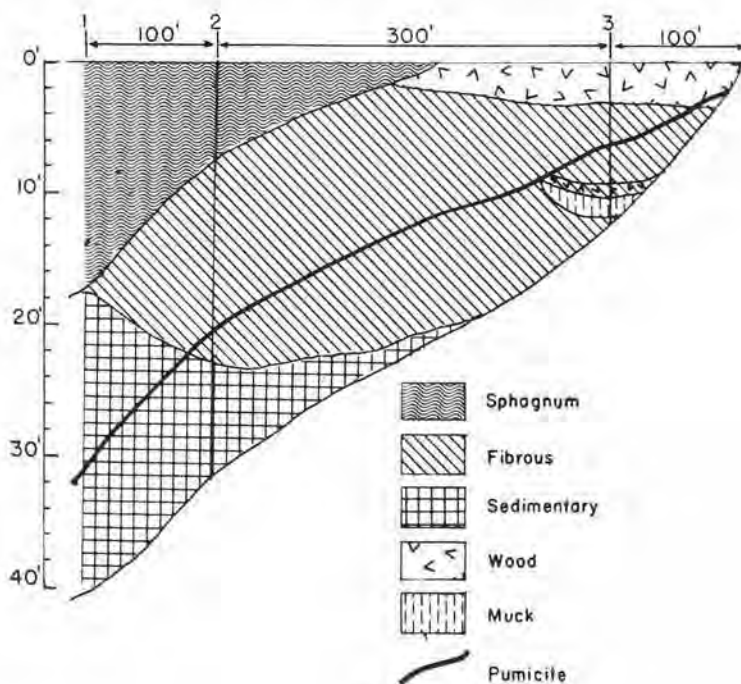
FIGURE 80.—Map and profile of Carpenter Lake peat area (102 acres). Map adapted from U. S. Department of Agriculture soil map of Kitsap County.
