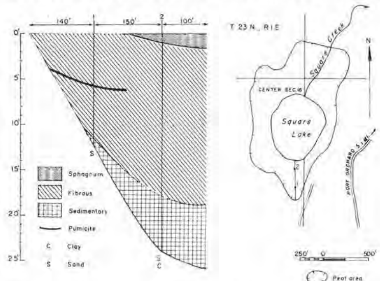
FIGURE 90.—Map and profile of Square Lake peat area (21 acres). Map adapted from U. S. Army Map Service photomosaic.
