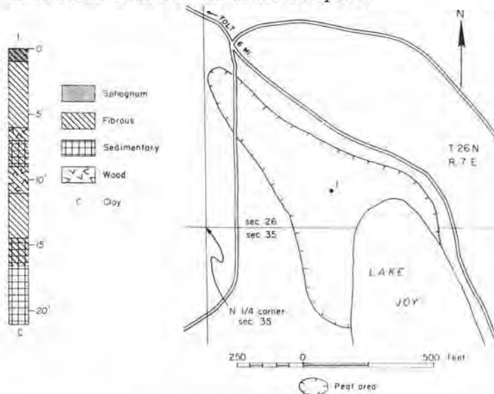
FIGURE 76.—Map and graphic log of a hole in Lake Joy peat area (6 acres). Map adapted from U. S. Department of Agriculture soil map of King County.
