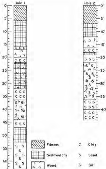
FIGURE 149.—Graphic logs of two holes north of Milton peat area No. 1.
