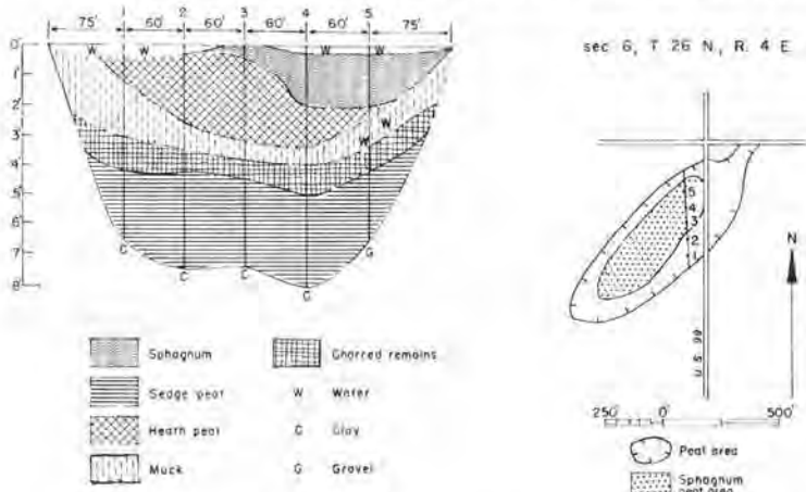
FIGURE 77.—Map and profile of Echo Lake peat area (5 acres). Map adapted from Rigg and Richardson (1938).
