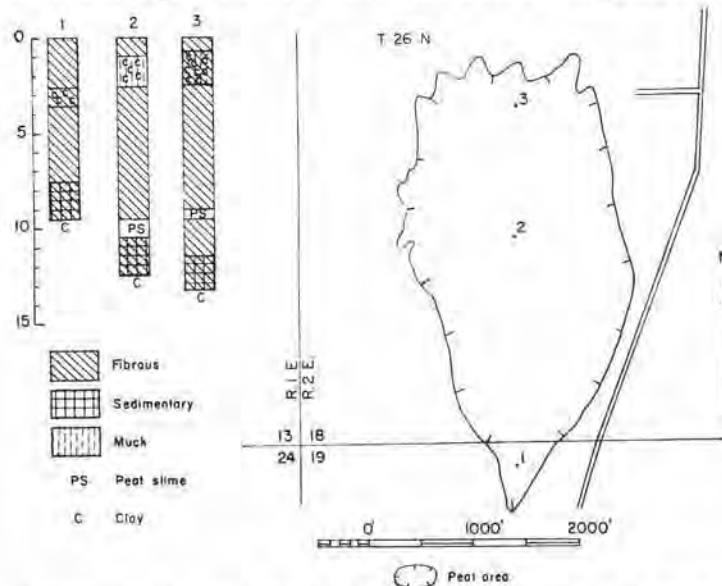
FIGURE 86.—Map and graphic logs of three holes in Port Madison Indian Reservation peat area (60 acres, estimated). Map adapted from U. S. Department of Agriculture soil map of Kitsap County.
