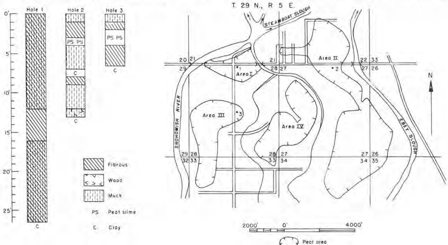
FIGURE 177.—Map and graphic logs of three holes in Ebey Island peat areas (932 acres). Map adapted from U. S. Department of Agriculture soil map of Snohomish County.
