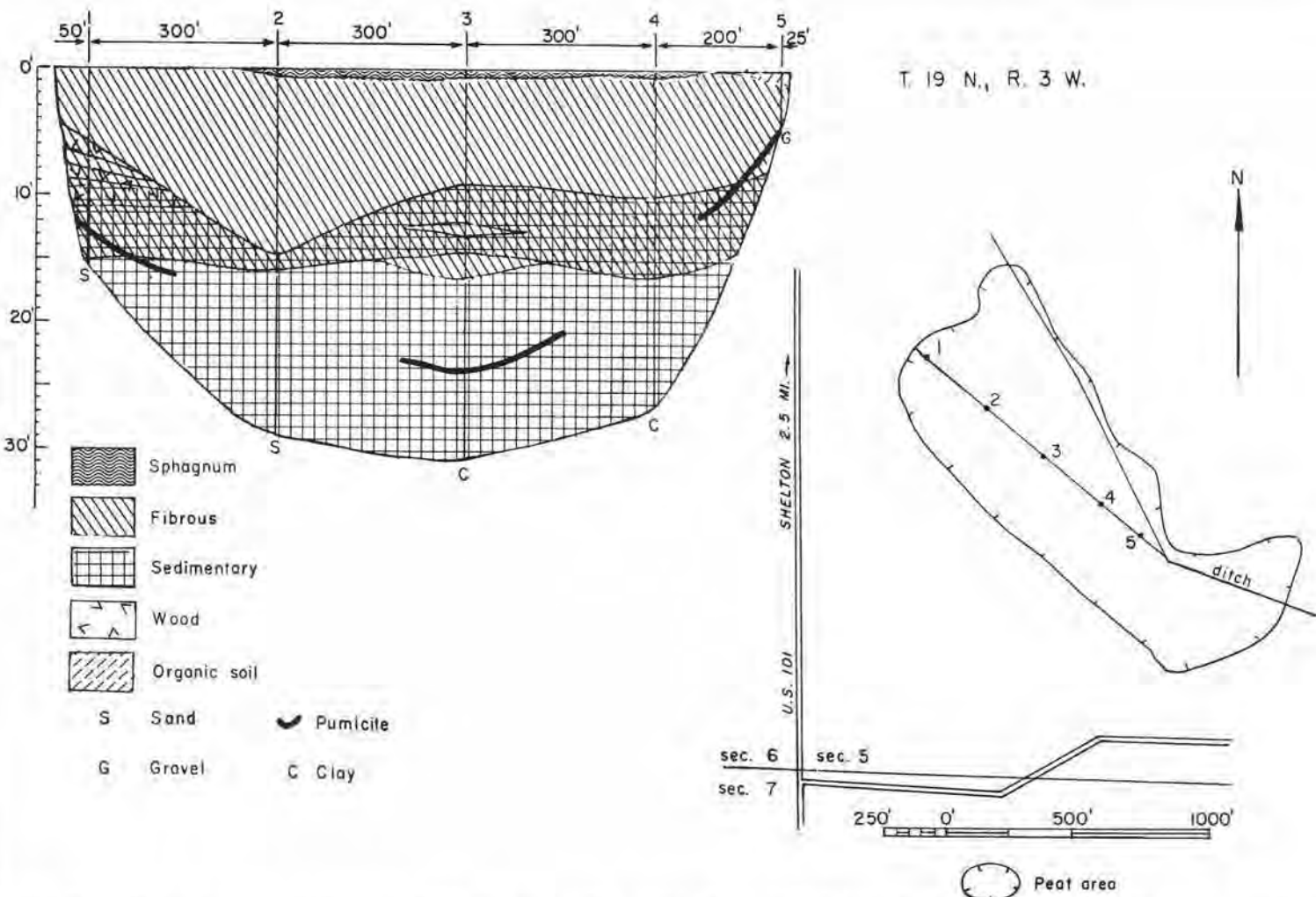
FIGURE 112.—Map and profile of Drainage Ditch peat area (23 acres). Map adapted from U. S. Department of Agriculture unpublished soil map of Mason County and U. S. Army Map Service photomosaic.
