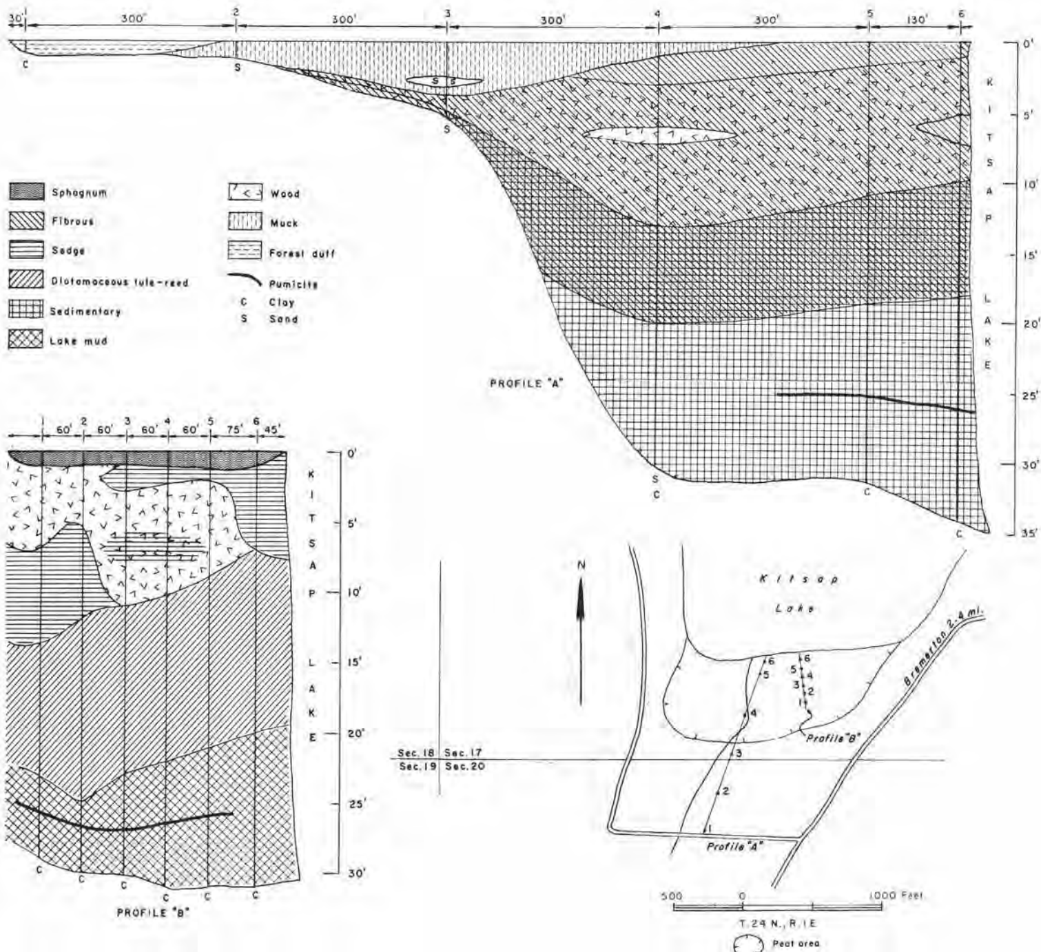
FIGURE 91.—Map and profiles of Kitsap Lake peat area (19 acres). Map adapted from U. S. Army Map Service photomosaic.
