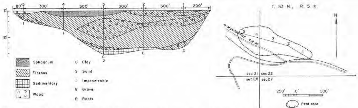
FIGURE 174.—Map and profile of Pilchuck Creek peat area (12 acres). Map adapted from U. S. Army Map Service photomosaic.
