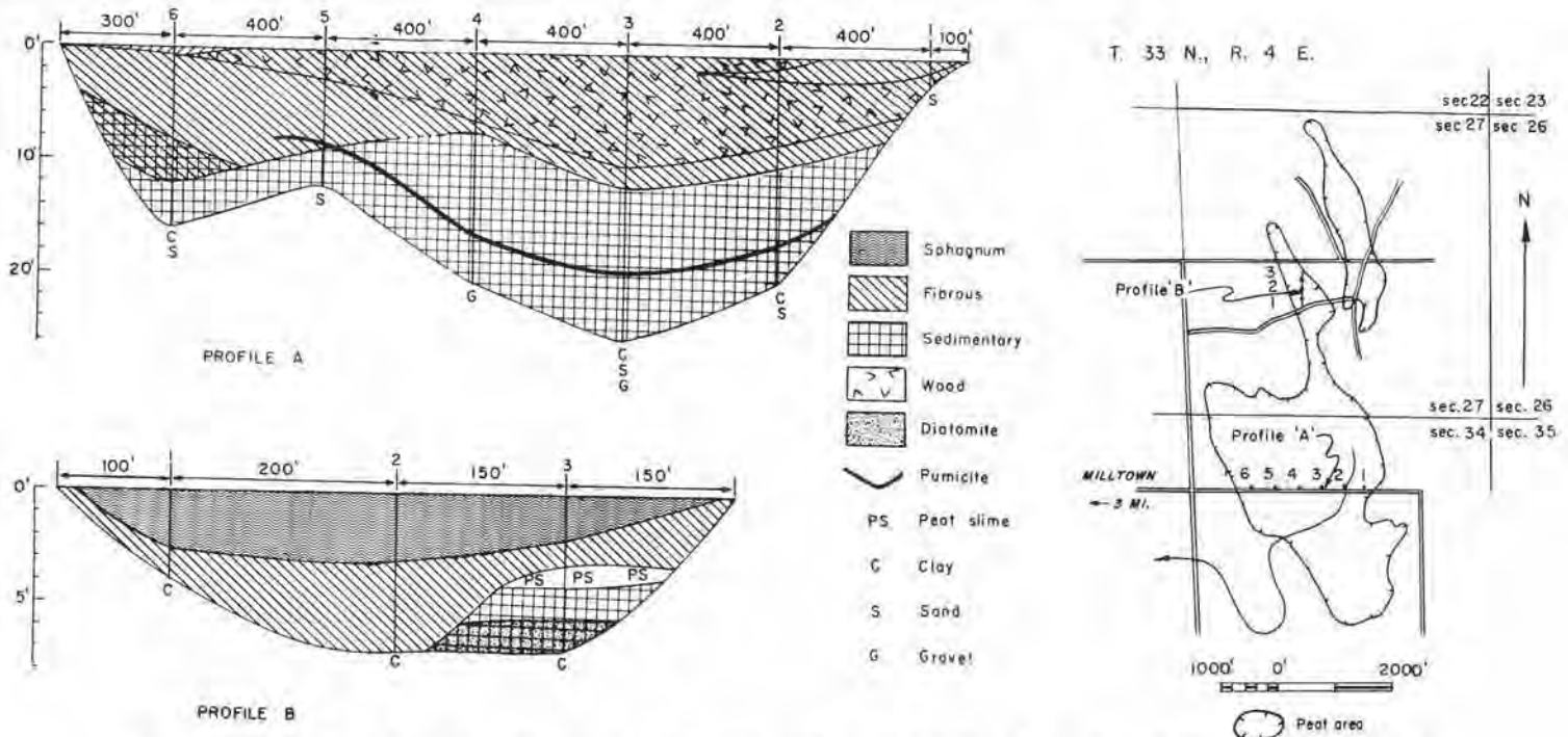
FIGURE 168.—Map and profiles of Milltown peat area (269 acres, including 3 acres of sphagnum). Map adapted from U. S. Soil Conservation Service soil map.
