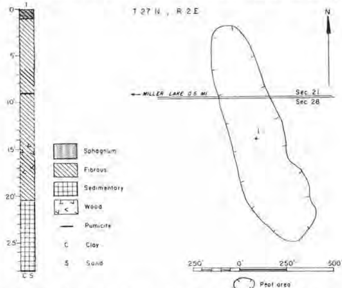
FIGURE 95.—Map and graphic log of a hole in Miller Lake peat area, Kitsap County (9 acres). Map adapted from U. S. Army Map Service photomosaic.
