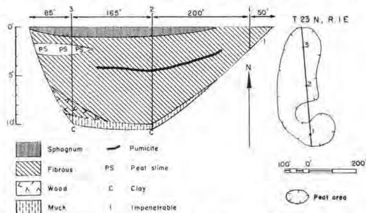
FIGURE 99.—Map and profile of Nels Johnson Lake peat area (2 acres). Map adapted from U. S. Department of Agriculture soil map of Kitsap County and U. S. Army Map Service photomosaic.
