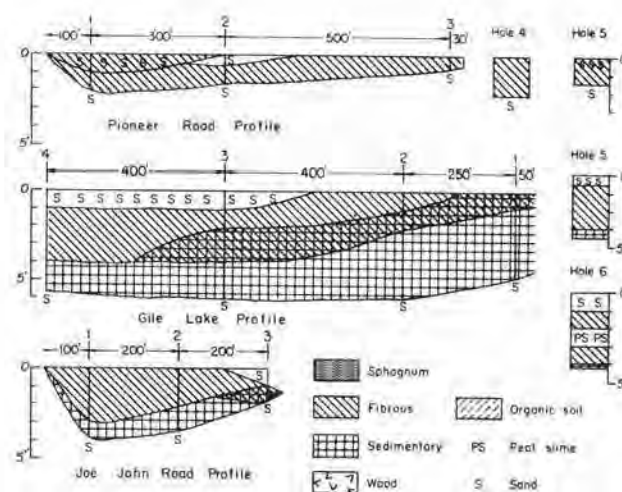
FIGURE 118.—Map and profiles of Peninsula peat areas, Pacific County (3,000 to 4,000 acres, estimated). Map adapted from U. S. Soil Conservation Service soil map and U. S. Army Map Service photomosaic.
