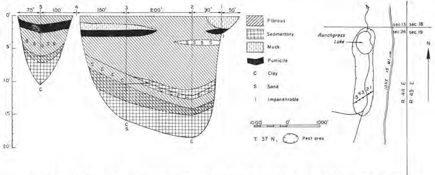
FIGURE 134.—Map and profile of Bunchgrass Meadow peat area (69 acres). Map adapted from U. S. Geological Survey topographic map (Metaline quadrangle).
