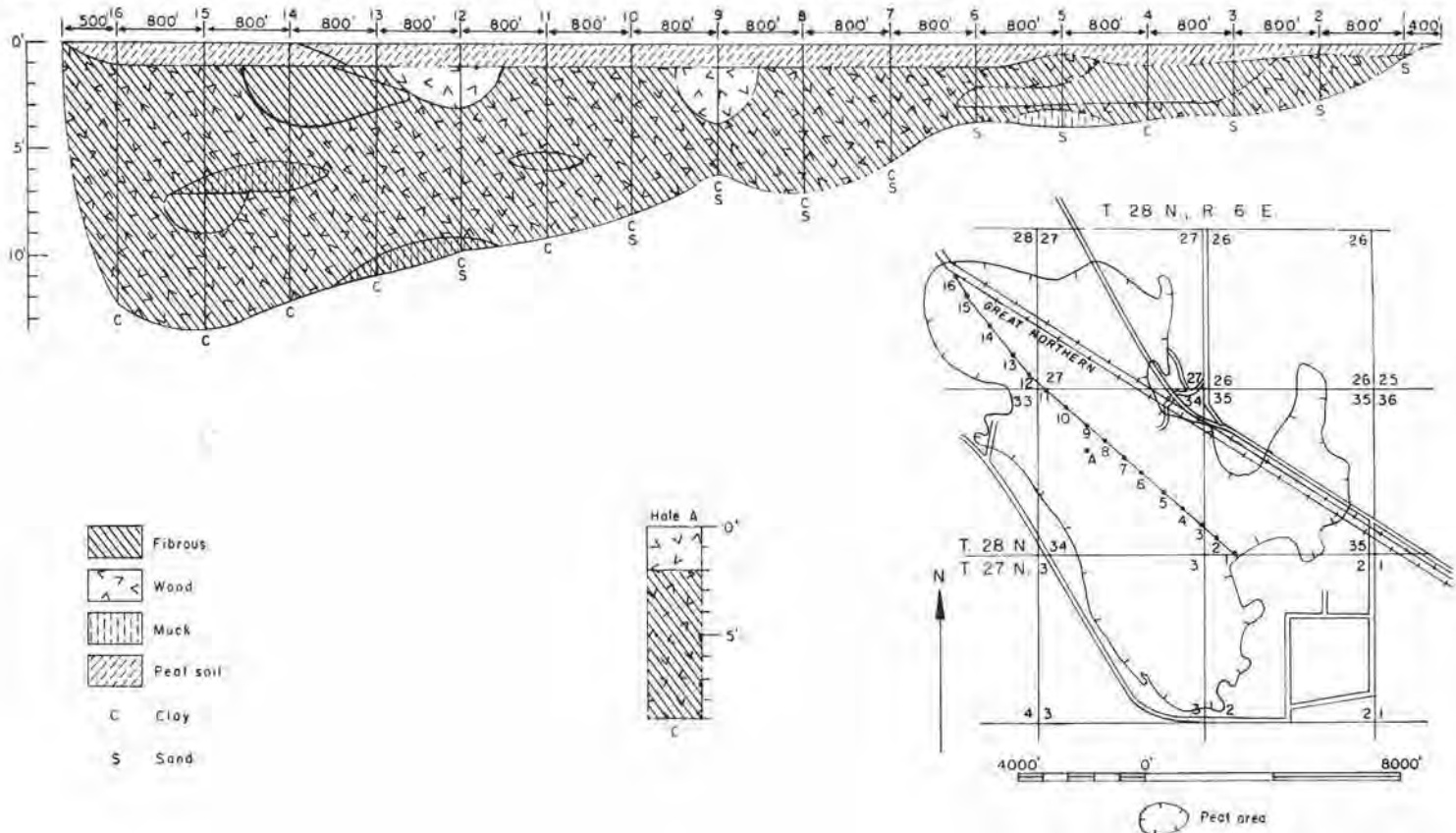
FIGURE 175.—Map, profile, and graphic log of a hole in Frye peat area (1,975 acres). Map adapted from U. S. Department of Agriculture soil map of Snohomish County.
