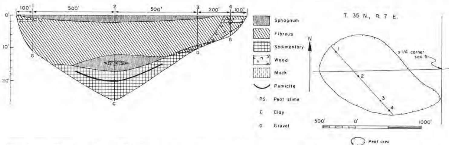
FIGURE 171.—Map and profile of Hamilton peat area (33 acres). Map adapted from U. S. Soil Conservation Service soil map.
