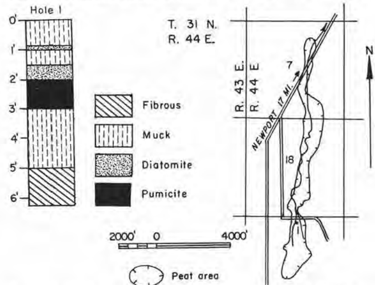
FIGURE 131.—Map and graphic log of a hole in Deer Creek peat area No. 1, Pend Oreille County (200 acres). Map adapted from aerial photograph.
