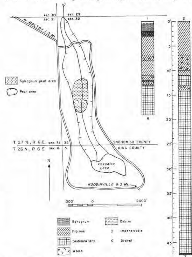
FIGURE 183.—Map and graphic logs of two holes in Paradise Lake peat area No. 2, Snohomish County (99 acres, including 17 acres of sphagnum). Map adapted from U. S. Department of Agriculture soil map of Snohomish County.
