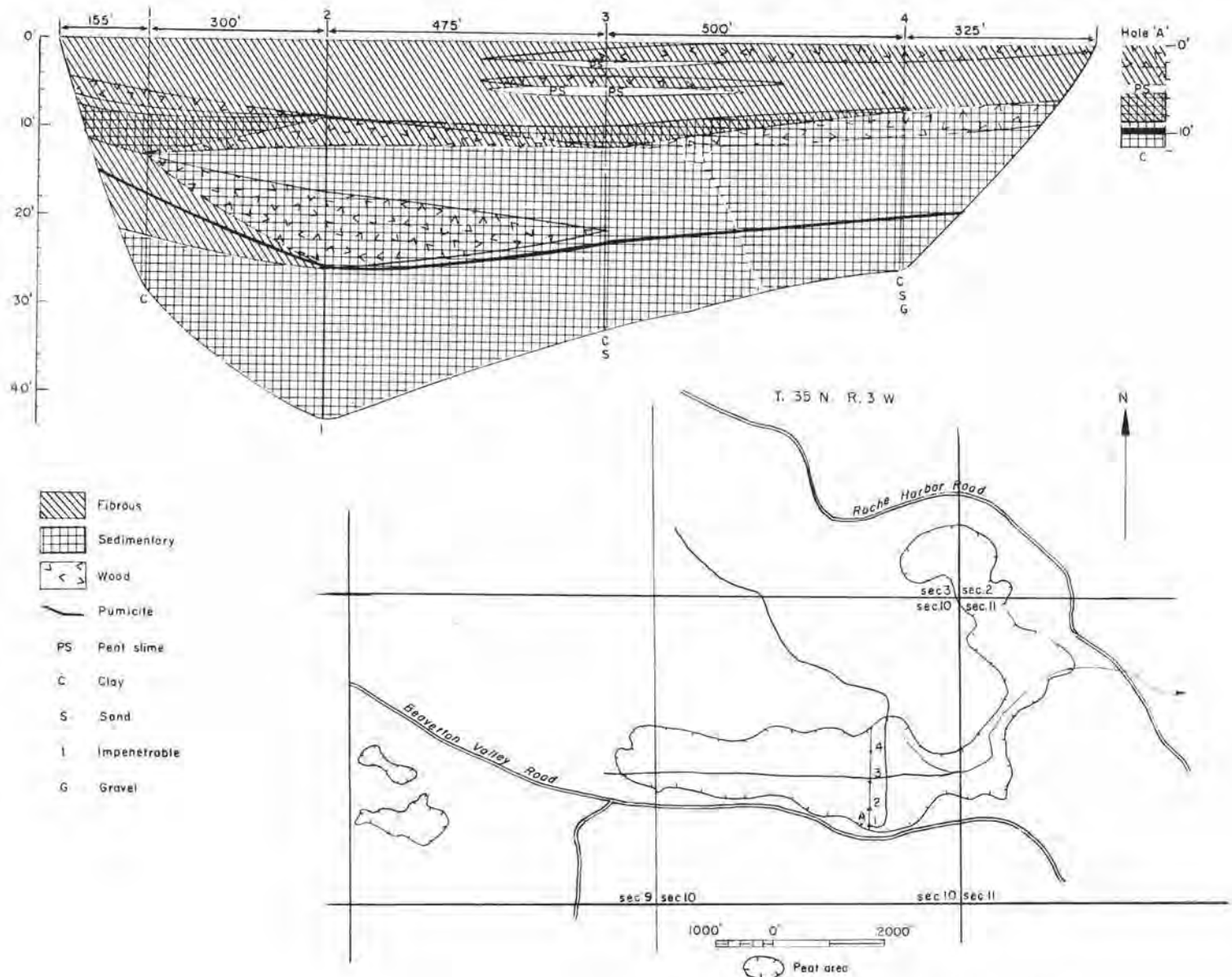
FIGURE 160.—Map, profile, and graphic log of a hole in Beaverton Valley peat area (240 acres). Map adapted from field sketch by John Sherman.
