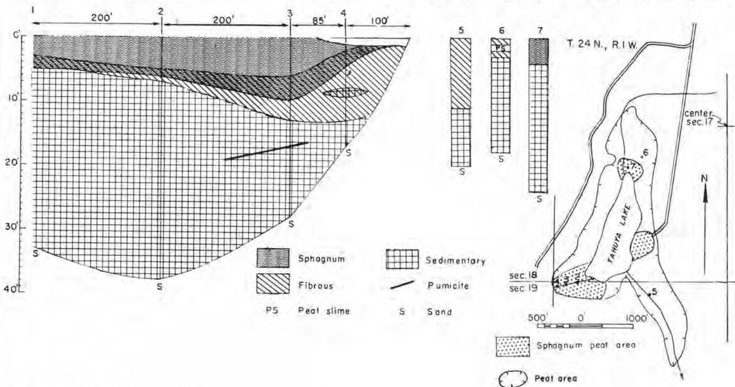
FIGURE 81.—Map, profile, and graphic logs of three holes in Tahuya Lake peat area (73 acres). Map adapted from U. S. Army Map Service photomosaic.
