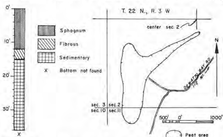
FIGURE 107.—Map and graphic log of a hole in Peninsula peat area, Mason County (40 acres). Map adapted from U. S. Department of Agriculture unpublished soil map of Mason County and U. S. Army Map Service photomosaic.
