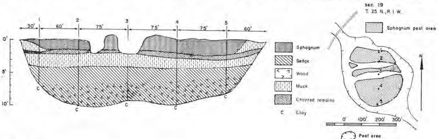
FIGURE 94.—Map and profile of Seabeck peat area (5 acres, estimated). Map adapted from Rigg and Richardson (1938) and U. S. Department of Agriculture soil map of Kitsap County.
