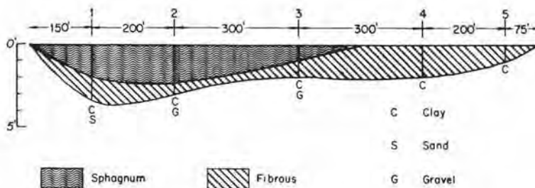
FIGURE 122.—Map and profile of Chinook peat area (45 acres). Map adapted from U. S. Army Map Service photomosaic.
