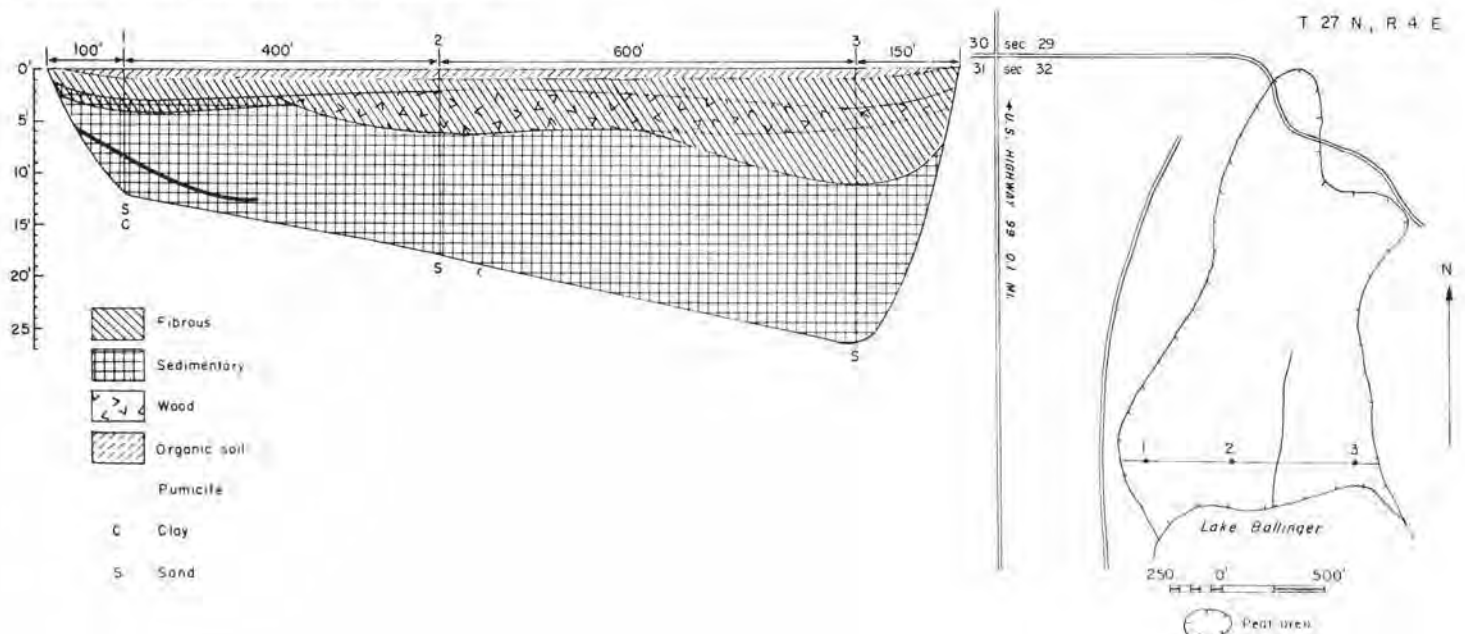
FIGURE 188.—Map and profile of Lake Ballinger peat area (41 acres). Map adapted from U. S. Army Map Service photomosaic.
