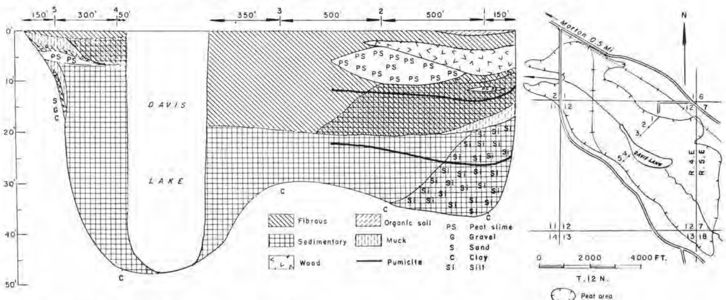
FIGURE 100.—Map and profile of Davis Lake peat area, Lewis County (542 acres). Map adapted from U. S. Department of Agriculture soil map of Lewis County.
