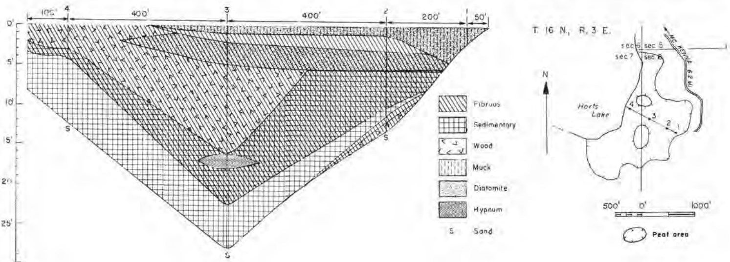
FIGURE 150.—Map and profile of Harts Lake peat area (43 acres). Map adapted from U. S. Department of Agriculture soil map of Pierce County.
