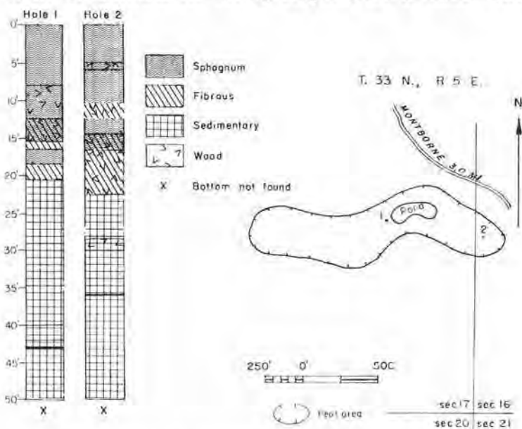
FIGURE 173.—Map and graphic logs of two holes in Big Lake peat area (12 acres). Map adapted from U. S. Army Map Service photomosaic.
