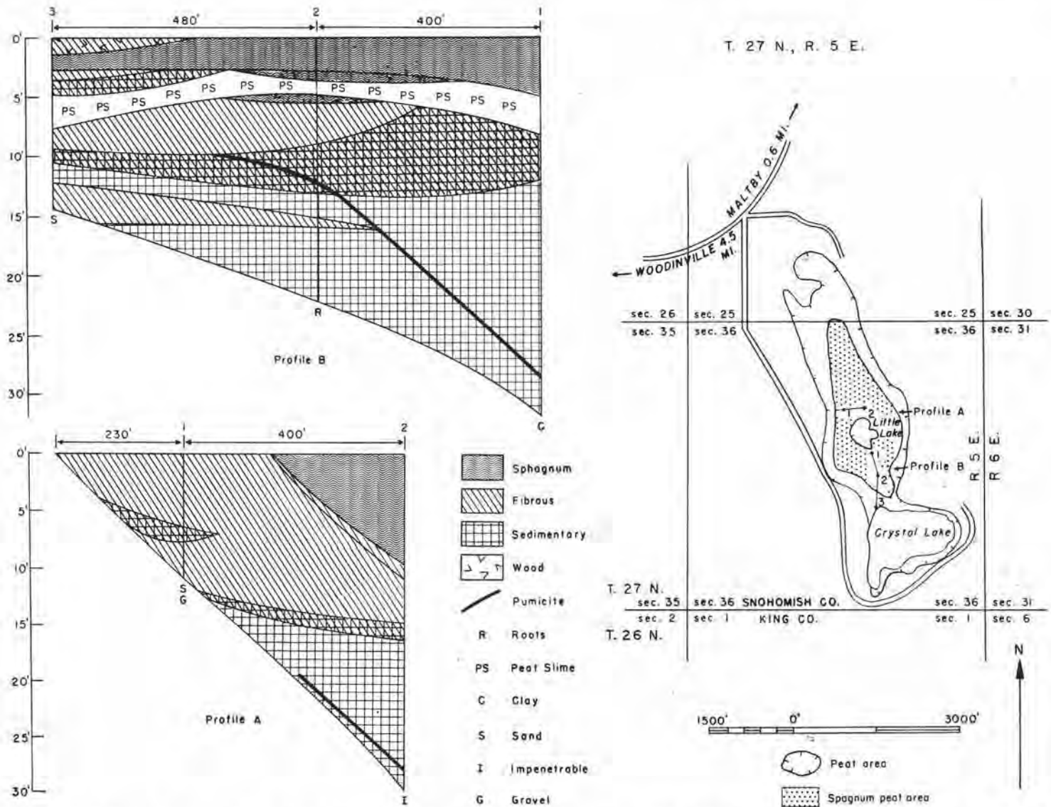
FIGURE 181.—Map and profiles of Crystal Lake-Little Lake peat area (133 acres, including 57 acres of sphagnum). Map adapted from U. S. Department of Agriculture soil map of Snohomish County.
