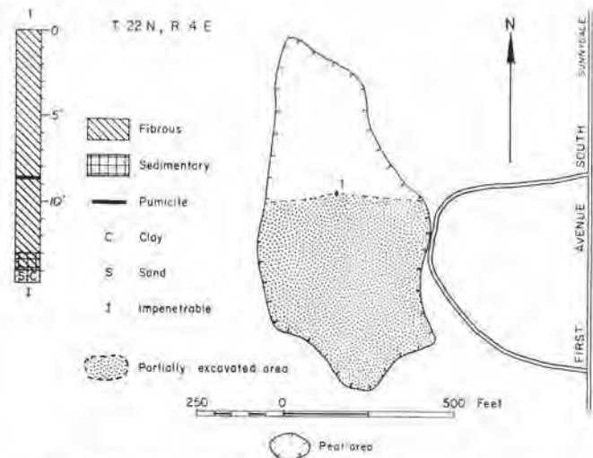
FIGURE 73.—Map and graphic log of a hole in Arrow Lake peat area (8 acres). Map adapted from U. S. Department of Agriculture soil map of King County and U. S. Army Map Service photomosaic.
