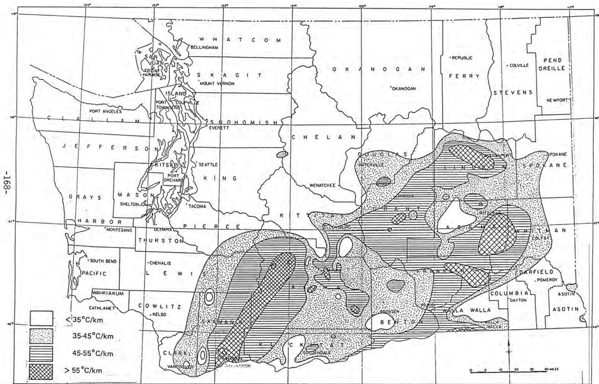
Figure 7-1. -- Temperature gradient contour map of Washington
