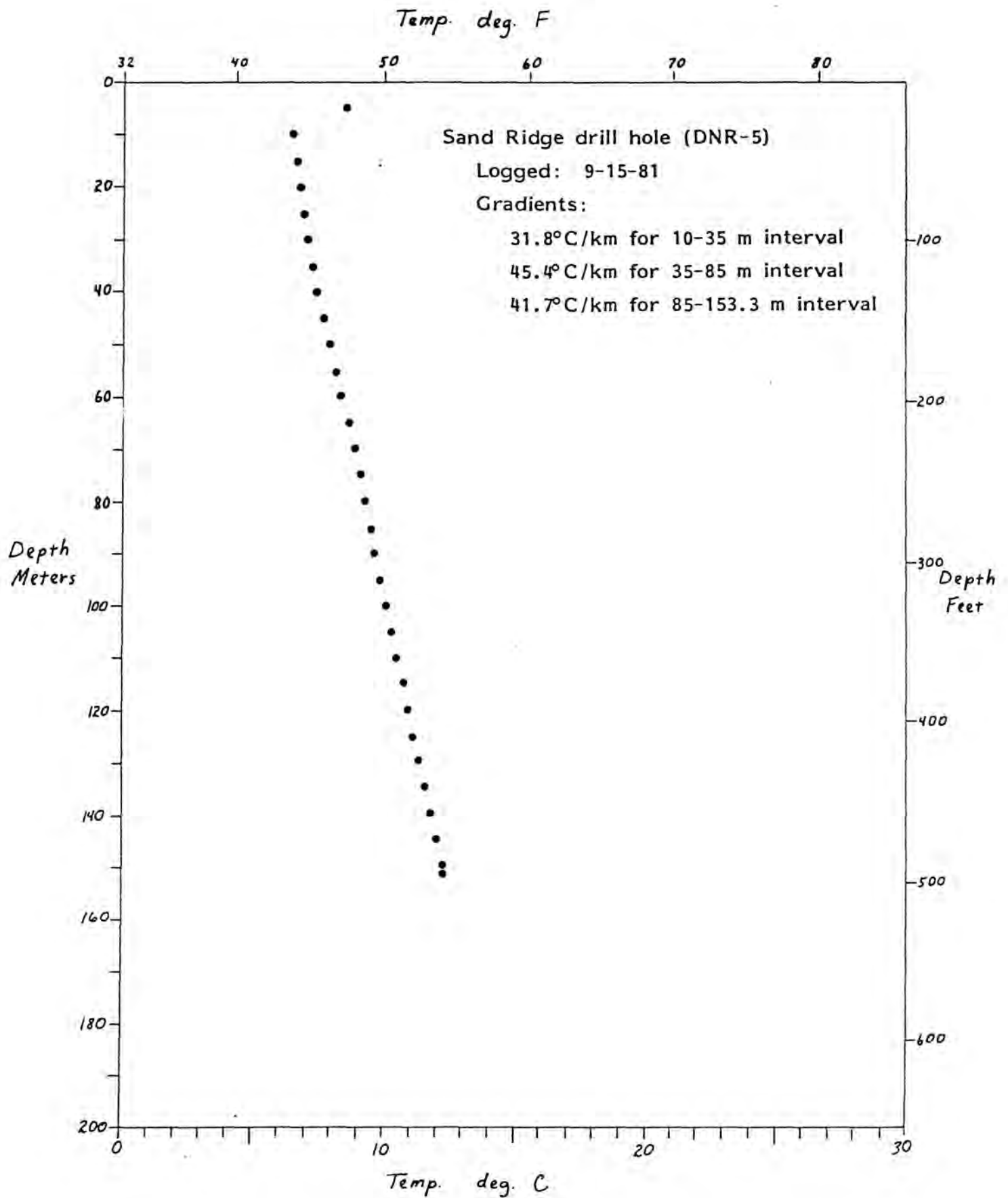
FIGURE 6-11.—Temperature-depth plot for Sand Ridge (DNR-5) drill hole.
