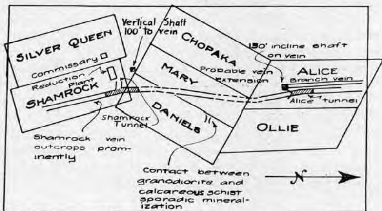
Fig. 19. Map showing claims and location of principal workings of the Four Metals Mine.
