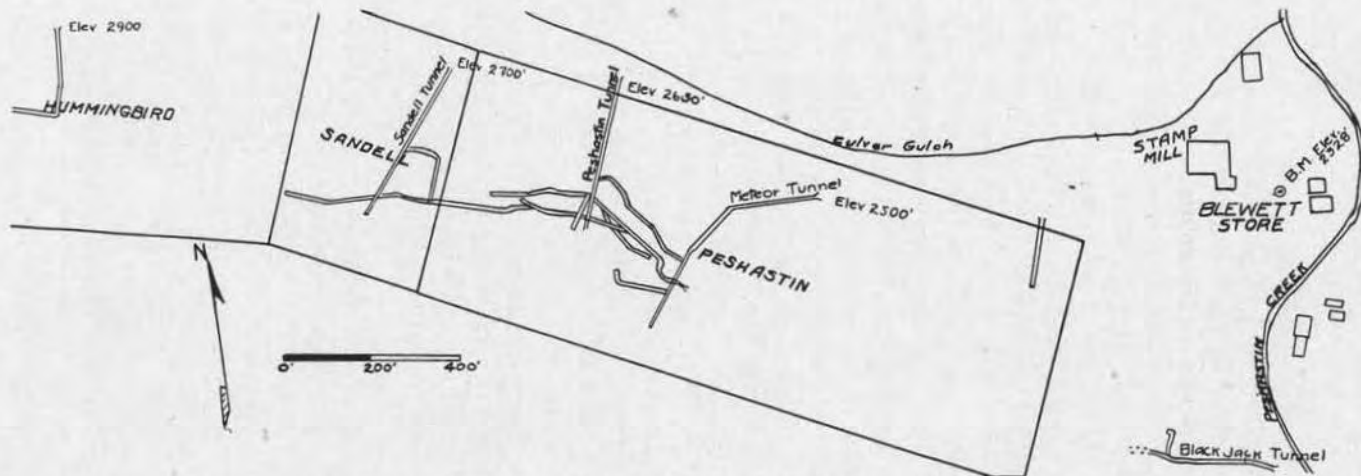
Fig. 22. Map showing mine workings on the east end of the Peshastin vein, near mouth of Culver Gulch, Blewett District.
