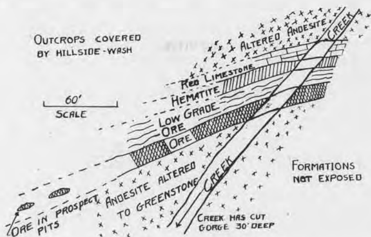
Fig. 27. Geologic sketch map of ore-body and associated formations at Apex Manganese Mine.
