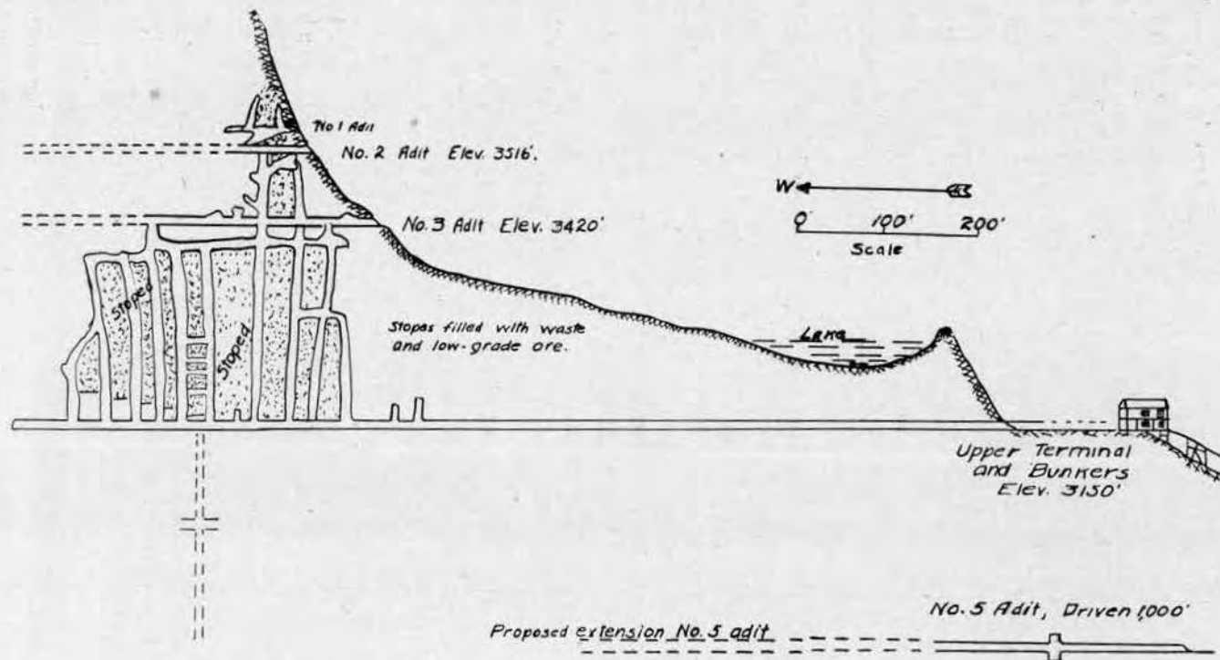
Fig. 25. Longitudinal section along plane of vein, to show development of Apex Gold Mine.
