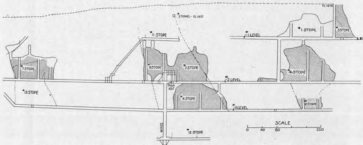
Fig. 24. Longitudinal section along plane of vein, to show development of Sunset Copper Mine, Index District.
