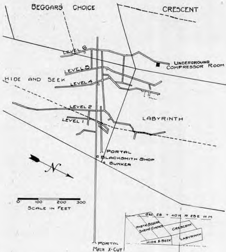
Fig. 20. Plan view of mine workings, Ruby Mine of Pyrargyrite Mining Company.
