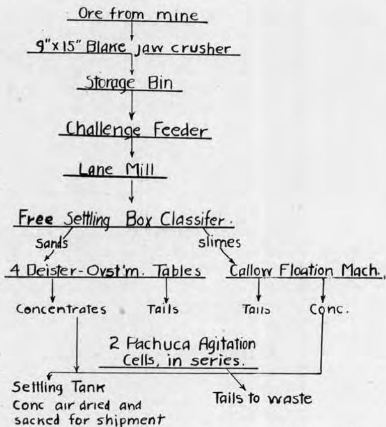
Fig. 17. Flow-sheet of the concentrator at the Phil Sheridan Mine.
