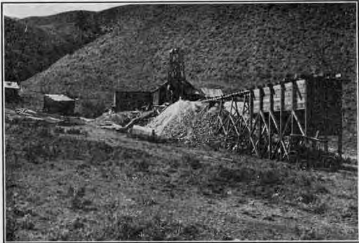
Head-frame and ore-bin, at Cabin shaft of Great Metals Mining & Milling Company.
