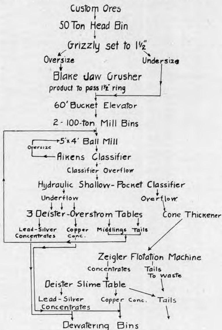
Fig. 18. Flow-sheet of the Bender Mill.
