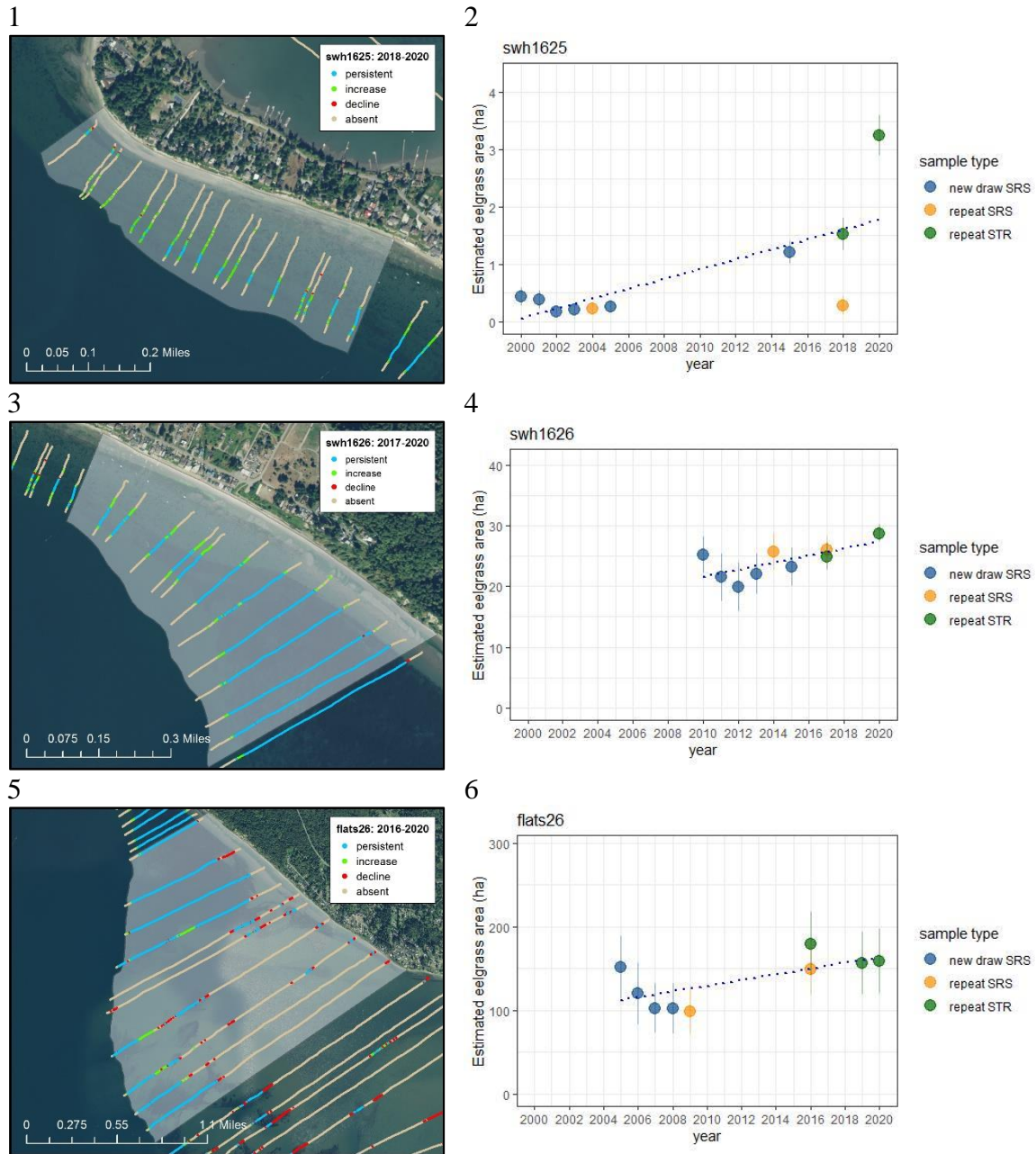
Figure 9: Change in eelgrass area over time at swh1625, swh1626 and flats26. The maps on the left side (1, 3, and 5) show where eelgrass appeared (green), disappeared (red), and was persistent over time (blue) along transects that were resampled over time. The years of the paired transect analysis are indicated on the map legends. The plots on the right show linear regression of all site samples over time. The different colors show the type of sample (new draw SRS, SRS repeat, or STR repeat). Error bars indicate standard error. The regression line is indicated in dark blue.
