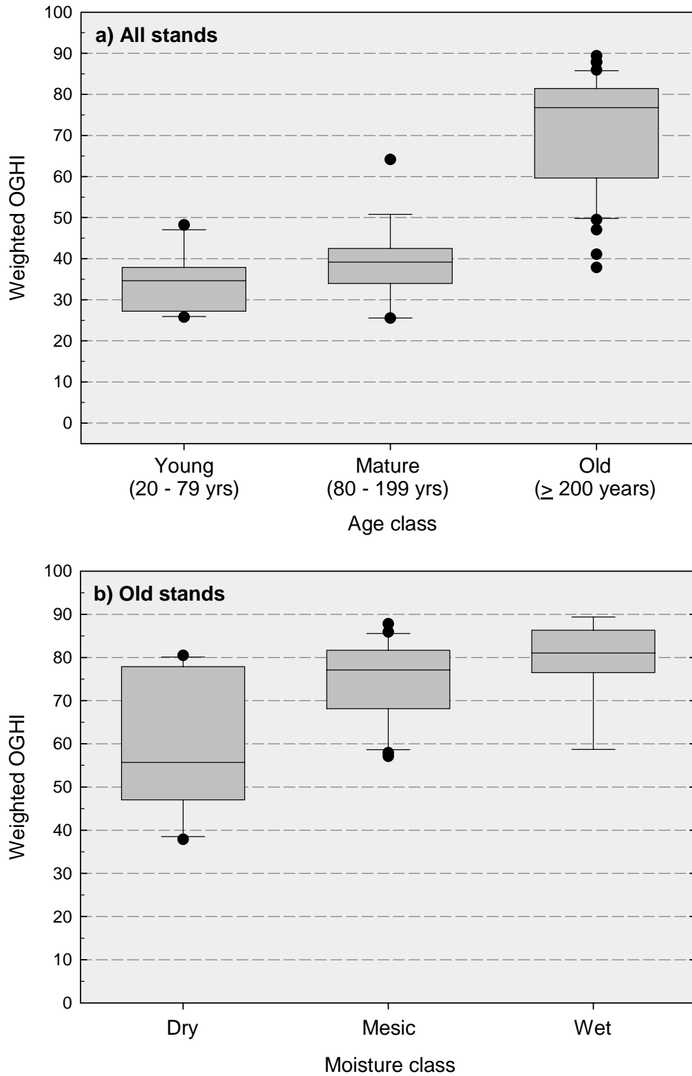
Figure 5. Box-and-whisker plots of weighted OGHl for a) all stands by age class, and b) old stands by moisture class.
